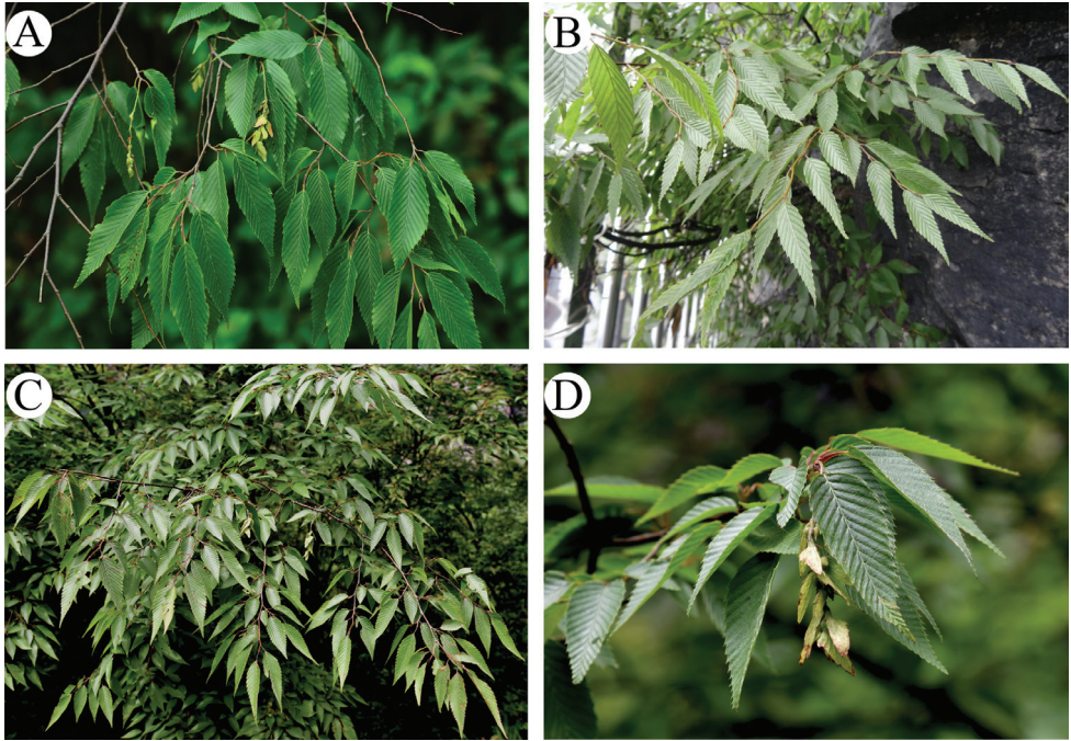
Figure 2. Carpinus polyneura A, B population from Tianmenshan, Zhangjiajie City (type locality of C. dayongina ) ( A photographed by H. Zhou B photographed by W. Q. Qin) C, D population from Wushan, Chongqing City (near the type locality of C. polyneura ) ( C, D photographed by H. L. Zhou).
