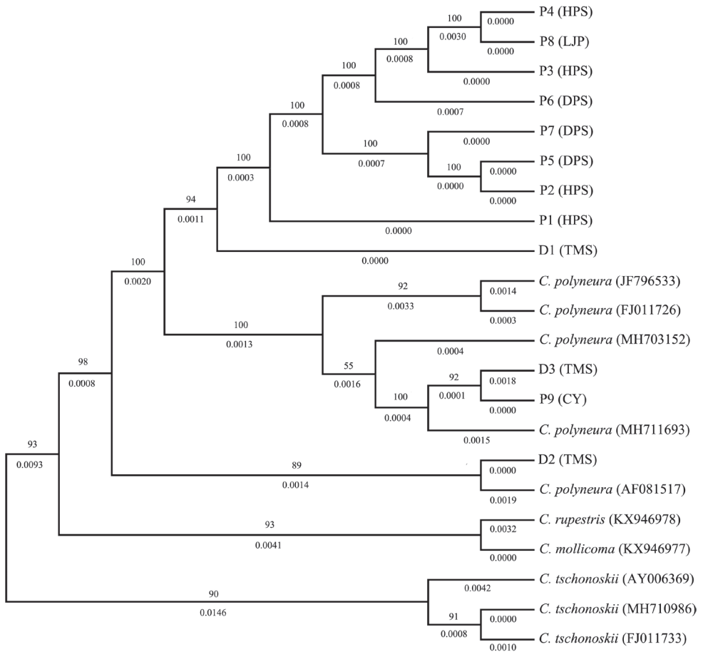
Figure 4. The neighbor-joining (NJ) tree, based on ITS sequence data. Carpinus mollicoma , C. rupestris and C. tschonokii as related species; P1–P4 are samples of C. polyneura from Hupingshan (HPS), Shimen, Hunan, China; P5–P7 are samples of C. polyneura from Dapanshan (DPS), Panan, Zhejiang, China; P8 is a sample of C. polyneura from Liujiaping (LJP), Wufeng, Hubei, China; P9 is a sample of C. polyneura from Caoyuan (CY), Longli, Guizhou, China; D1–D3 are samples of C. dayongina from Tianmenshan (TMS), Zhangjiajie, Hunan, China. The numbers above the branch are bootstrap values (%), and the numbers below the branch are branch length.
