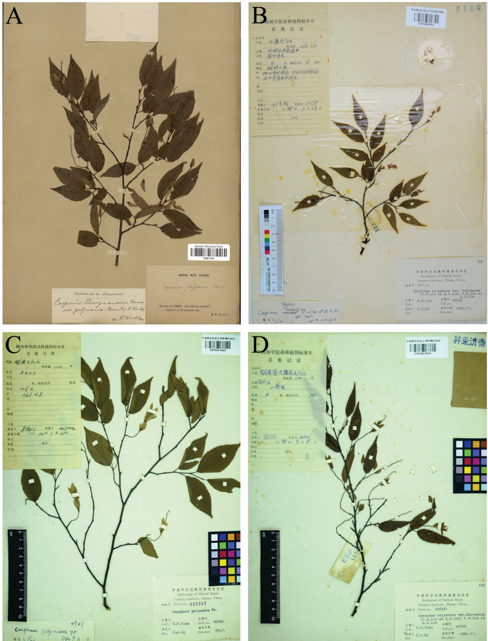
Figure 1. Specimens of Carpinus polyneura Franchet A lectotype of C. polyneura (P. G. Farges s.n., P06811144) B holotype of C. dayongina K. W. Liu & Q. Z. Lin (K. W. Liu 33359, CSFI050241) C paratype of C. dayongina (Y. T. Xiao 40700, CSFI017465) D paratype of C. dayongina (Y. T. Xiao 40700, CSFI017535).
