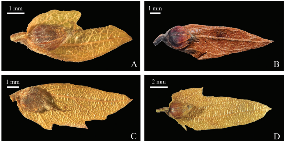
Figure 3. Nutlet trichomes of C. polyneura A from isotype of C. dayongina (K. W. Liu 33359, PE01843387) B from paratype of C. dayongina (Y. T. Xiao 40700, CSFI017539) C from T. L. Dai 104469, PE00818275 D from W. P. Fang 7546, PE00818253. A, C, D photographed by Q. Q. He B photographed by X. Li.
