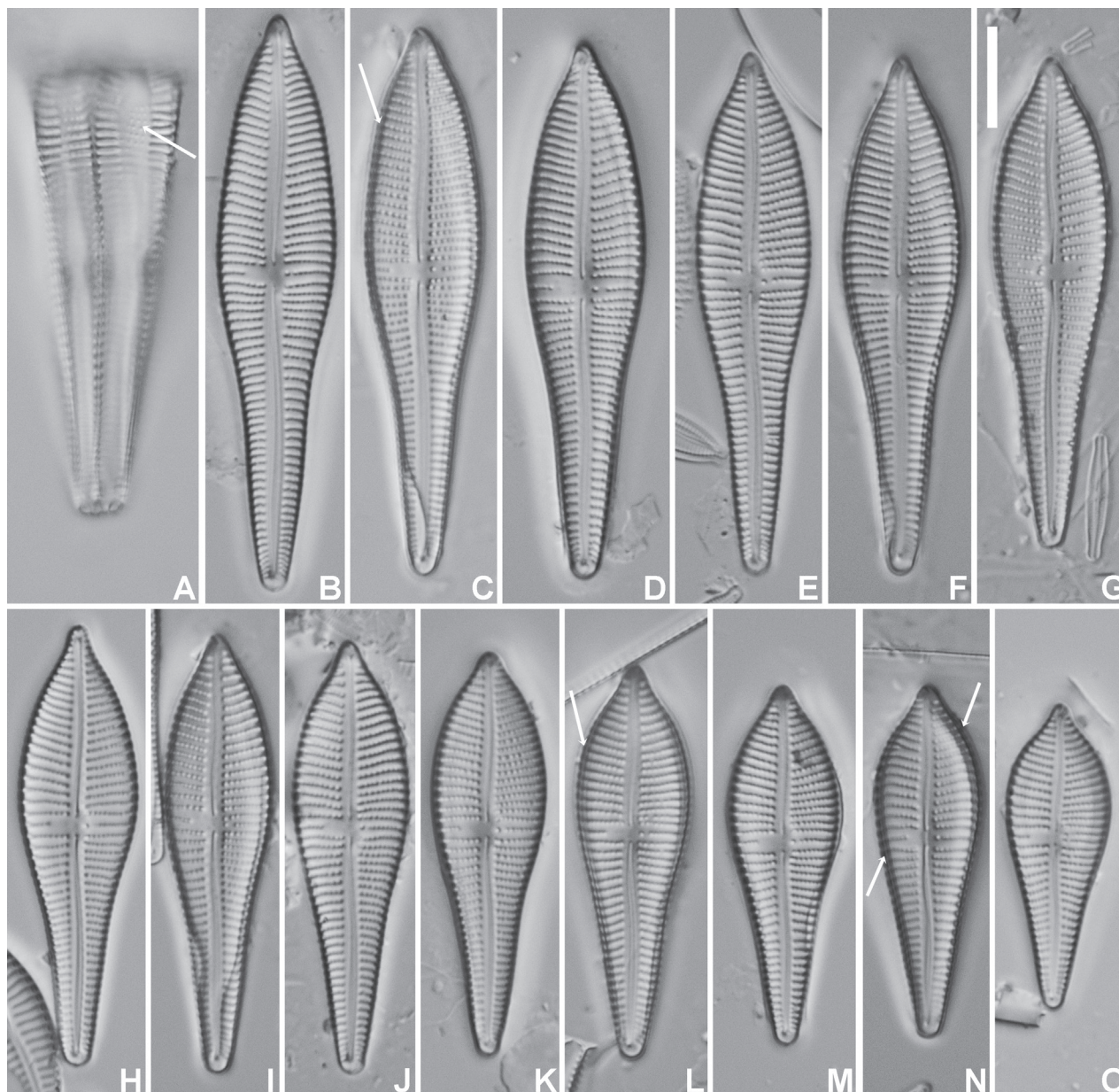
Figure 1. Gomphonema vancampianum sp. nov. LM micrographs taken from the holotype material (BR-4839, Lac du Drapeau, Sample DRAPEAU-U03VEG, France) A LM picture of a frustule in girdle view. The arrow indicates the smaller, more distantly spaced areolae on the mantle B–O LM pictures of valves in valve face view in decreasing length. The arrows indicate the possible presence of the marginal crest. Scale bar: 10 \mu m.
