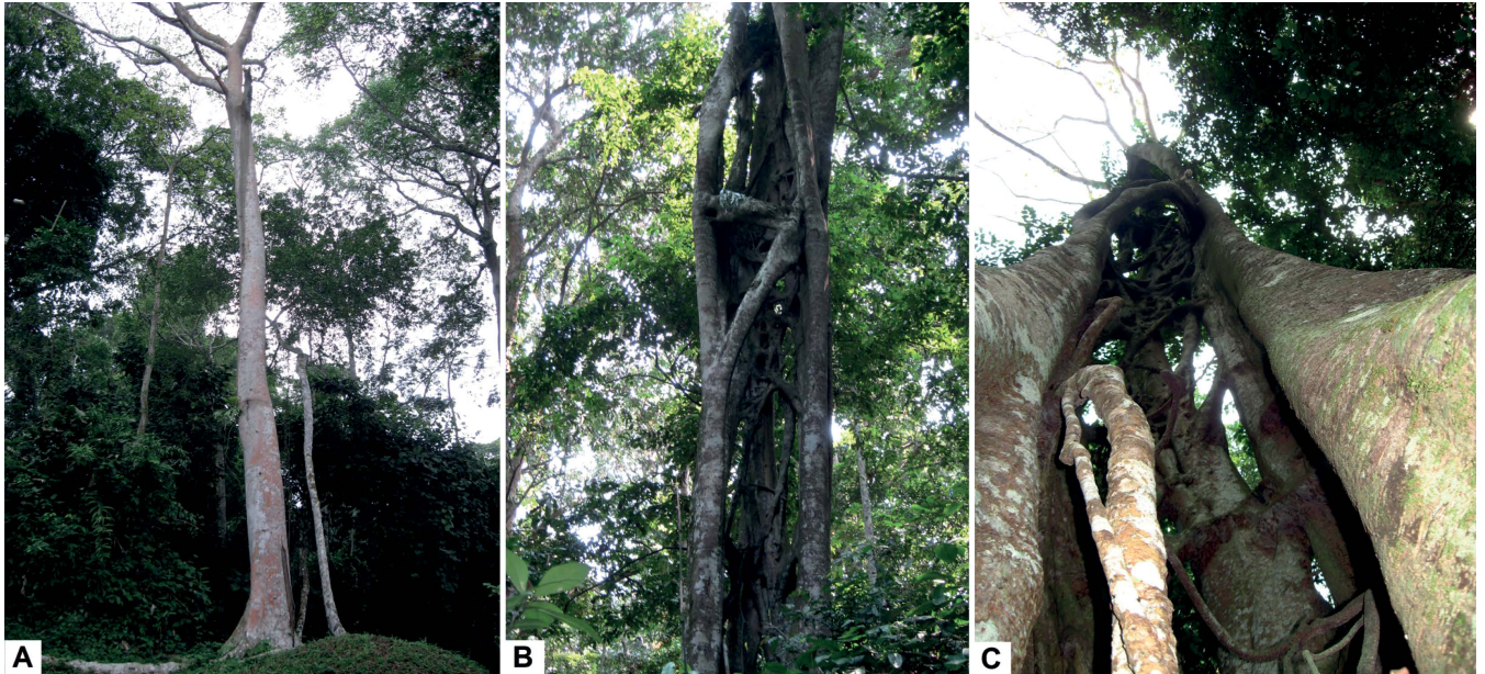
Figure 2 – Trunk v. pseudo-trunk in a tree and a hemi-epiphyte: A, true trunk of the tree Ficus mucoso Ficalho; B, pseudo-trunk of the hemi-epiphyte F. recurvata De Wild. seen from the side; C, and from inside and below in a different individual.
