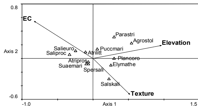
Figure 1 – CCA-ordination biplot based on the new salt marsh relevés (the arrows show the environmental variables; EC = electric conductivity, as a proxy of salinity; Texture = median of particle size). Only the more frequent and/or most abundant and typical salt-marsh species are shown. (Agrostol = Agrostis stolonifera , Atrilitt = Atriplex littoralis , Atripros = Atriplex prostrata , Elymathe = Elymus athericus (in some rare cases also E. repens occurred on the new marsh, it is included within Elymathe), Parastr = Parapholis strigosa , Plancore = Plantago coronopus , Puccmari = Puccinellia maritima , Salieuro = Salicornia europaea , Salipro = Salicornia procumbens , Salskali = Salsola kali , Spersali = Spergularia marina , Suaemari = Suaeda maritima ).
