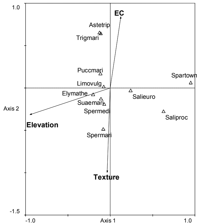
Figure 2 – CCA-ordination biplot based on the old salt marsh relevés (the arrows show the environmental variables; EC = electric conductivity, as a proxy of salinity; Texture = median of particle size). Only the more frequent and/or most abundant and typical salt-marsh species are shown. (Astetrip = Aster tripolium , Elymathe = Elymus athericus , Limovulg = Limonium vulgare , Puccmari = Puccinellia maritima , Salieuro = Salicornia europaea , Saliproc = Salicornia procumbens , Spartown = Spartina townsendii , Spermedi = Spergularia media , Spermari = Spergularia marina , Suaemari = Suaeda maritima , Trigmari = Triglochin maritimum ).
