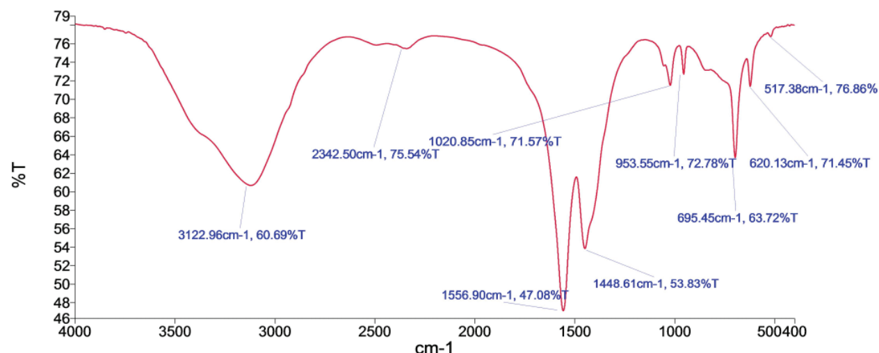
Figure 5. FTIR Spectrum of TA-AgNPs.
