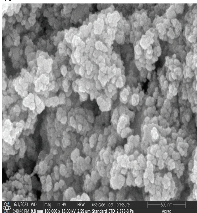
Figure 2. FESEM results of TA-AgNPs: A. SEM imaging; B. Mean average size.
