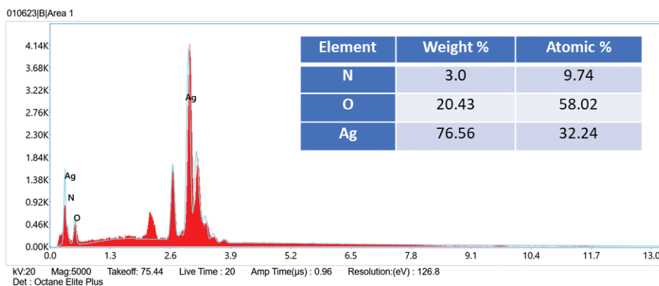
Figure 3. EDX Spectra of TA-AgNPs.
