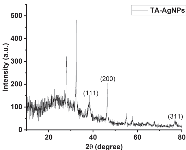
Figure 4. XRD Spectrum of TA-AgNPs.
