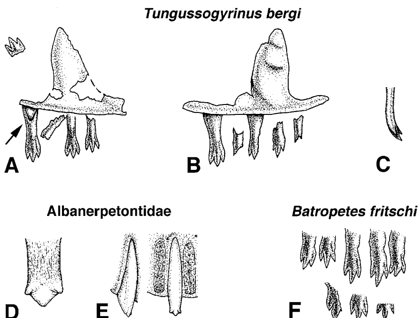
Figure 10. Dentition of branchiosaurids ( A–C ), albanerpetontids ( D–E ) and microsaurids ( F ). A–C. Tricuspid teeth in Tungussogyrinus bergi ; A. Premaxilla, PIN 4262/4a, note the isolated tricuspid crown, perhaps a hint of pedicel; B. Premaxilla PIN 4262/1b; C. Premaxillary tooth in distal and slightly lingual views; D. One tooth of the dentary of Anoualerpeton priscus Gardner et al., 2003. (drawn after a photograph in Gardner et al. 2003); E. Premaxillary tooth (inverted) in lingual and distal slightly lingual views of Albanerpeton inexpectatum Estes and Hoffstetter, 1976 (drawn after Gardner 2001); F. Tricuspid teeth of the dentary (above) and premaxilla in Batropetes fritschi (Geinitz & Deichmüller, 1882), NHMM-PW 2001/309-LS (drawn after a photograph from K. Krätschmer).
