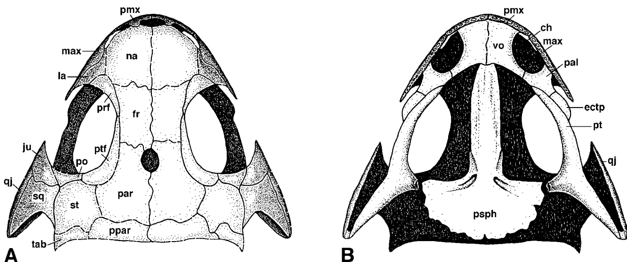
Figure 1. Tungussogyrinus bergi Efremov, 1939, reconstruction of skull, using a composite of several specimens (PIN 4262/1a, 6a, b, 7a, b, 9a, b). A. Dorsal view; B. Palatal view; skull length 9.2 mm. Abbreviations: ch – choana; ectp – ectopterygoid; fr – frontal; ju – jugal; la – lacrimal; max – maxilla; na – nasal; pal – palatine; par – parietal; pmx – premaxilla; po – postorbital; ppar – postparietal; prf – prefrontal; psph – parasphenoid; pt – pterygoid; ptf – postfrontal; qj – quadratojugal; sq – squamosal; st – supratemporal; tab – tabular; vo – vomer.
