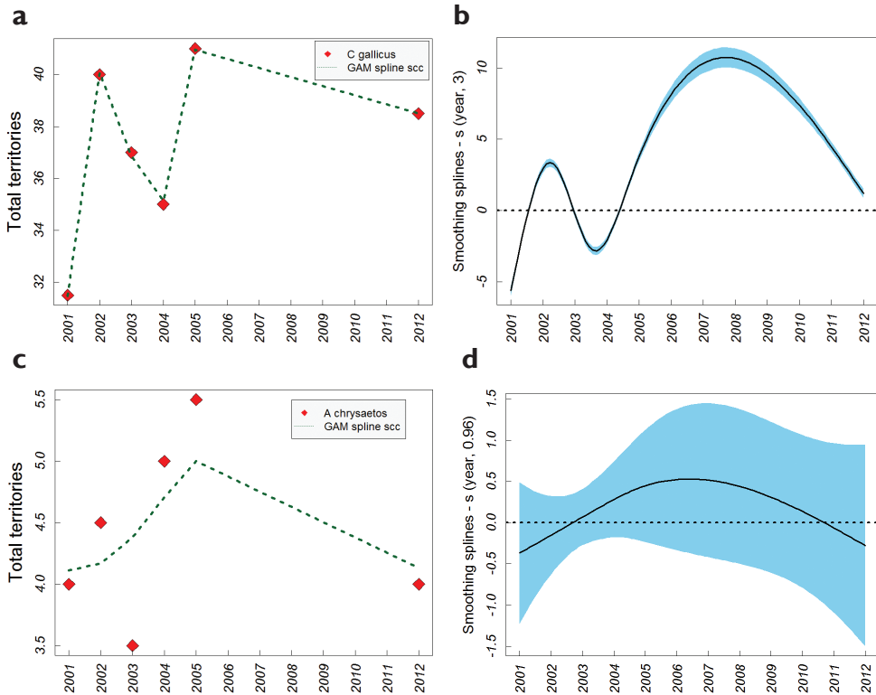
Figure 7. Inter-annual variation in the numbers of territories for Short-toed eagle and Golden eagle in Dadia-Lefkimi-Souffi National Park fitting Generalised Additive Models. Population trend modelling is also shown for each species, with cyclic cubic regression (cc) splines used as smoothing terms. a Variation in the number of Short-toed eagle territories fitting a GAM b Predictive GAM for the Short-toed eagle with smoothed terms (cc splines) c Variation in the number of Golden eagle territories fitting a GAM d Predictive GAM for the Golden eagle with smoothed terms (cc splines).
