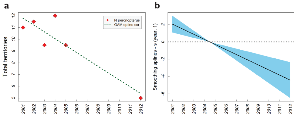
Figure 12. Inter-annual variation in the number of Egyptian vulture in Dadia-Lefkimi-Souffi National Park fitting Generalised Additive Models. Population trend modelling is also shown for the species with cubic regression (cr) splines used as smoothing terms. a Variation in the number of Egyptian vulture territories fitting a GAM b Predictive GAM for the Egyptian vulture with smoothed terms (cr splines).
