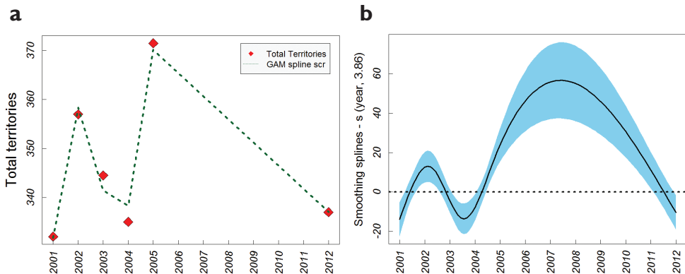
Figure 13. Inter-annual variation in the number of overall raptor territories in Dadia-Lefkimi-Souffi National Park fitting Generalised Additive Models. Population trends modelling is also demonstrated for the whole number of territories with cubic regression (cr) splines used as smoothing terms. a Variation in the number of overall raptor territories fitting a GAM b Predictive GAM for overall raptor territories with smoothed terms (cr splines).
