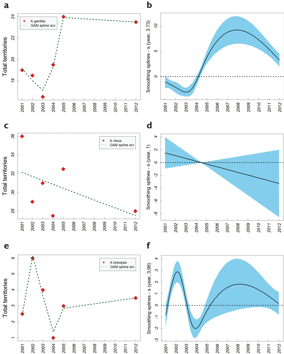
Figure 10. Inter-annual variation in the number of hawk territories in Dadia-Lefkimi-Souffi National Park fitting Generalised Additive Models. Population trend modelling is also shown for each species with cubic regression (cr) or cyclic cubic regression (cc) splines used as smoothing terms, depending on lowest AIC in each case. a Variation in the number of Northern goshawk territories fitting a GAM b Predictive GAM for the Northern goshawk with smoothed terms (cc splines) c Variation in the number of Eurasian sparrowhawk territories fitting a GAM d Predictive GAM for the Eurasian sparrowhawk with smoothed terms (cr splines) e Variation in the number of Levant sparrowhawk territories fitting a GAM f Predictive GAM for the Levant sparrowhawk with smoothed terms (cr splines).
