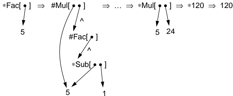
Fig. 1.(b) An evaluation of \text{Fac}[5]
