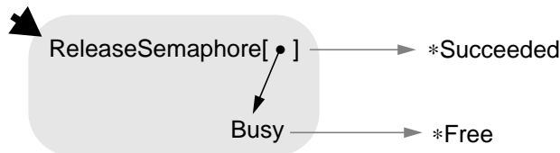
Fig. 2.(c) Rule for releasing a semaphore.
