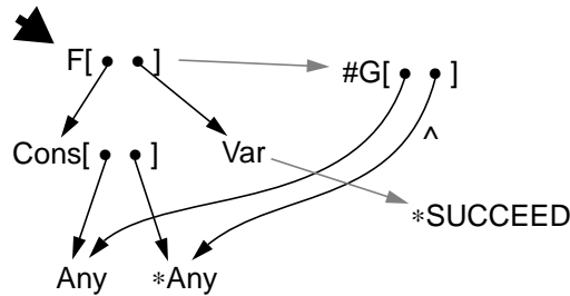
Fig. 4 A rule.
