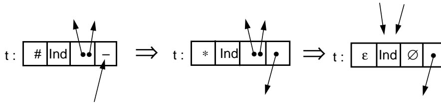
Fig. 17 Notification via a suspended Ind.
