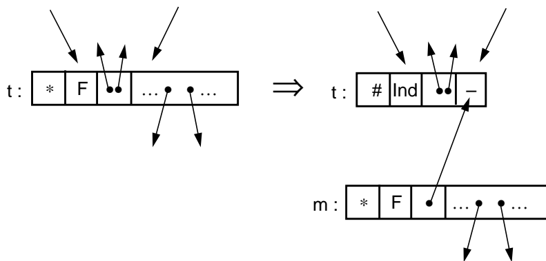
Fig. 16 Volatilising a non-volatile active packet
