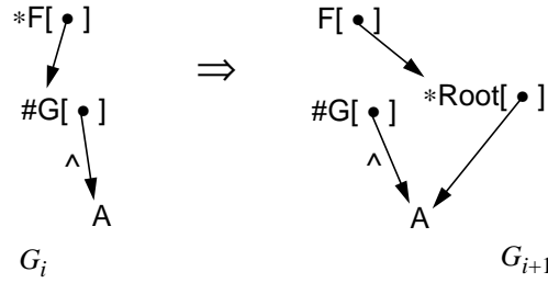
Fig. 9 A garbage node becomes live.
