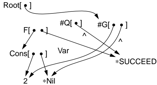
Fig. 7 Activation.
