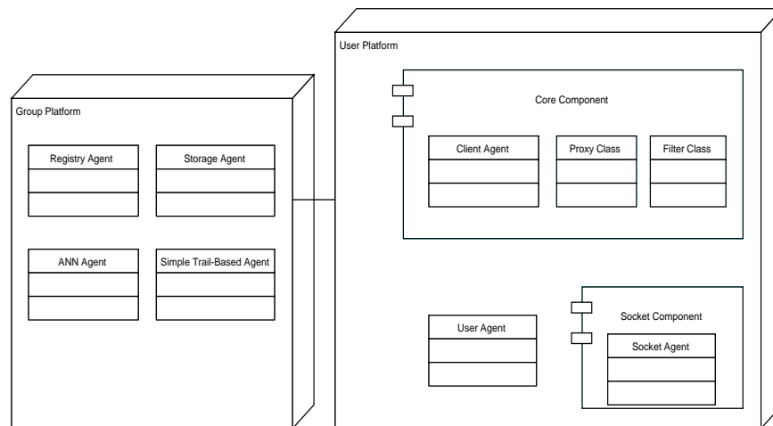
Figure 1: Framework architecture
