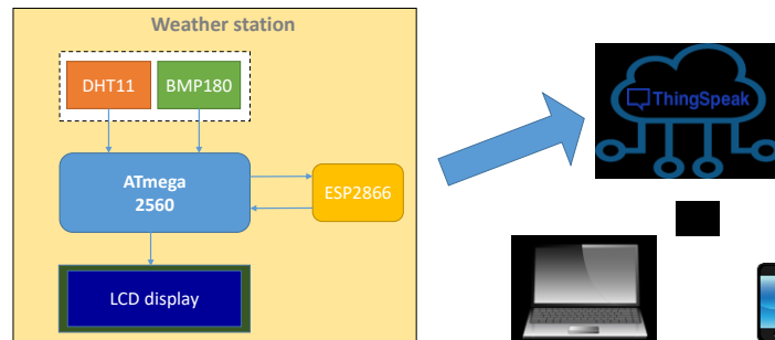
Figure 7: Weather Station block scheme
