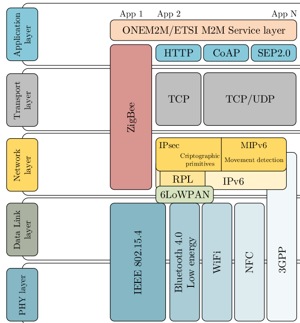
Figure 3: The overview of IoT standards in network layer architecture
