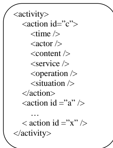
Figure 8: Data structure
