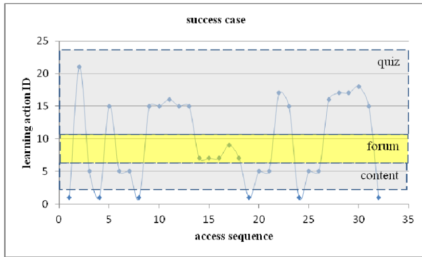
Figure 10: Success case
