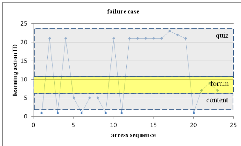
Figure 11: Failure case
