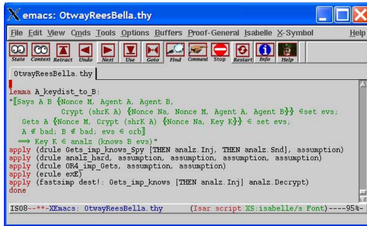
Figure 3: Proving key distribution for A in the Otway-Rees-Bella protocol
