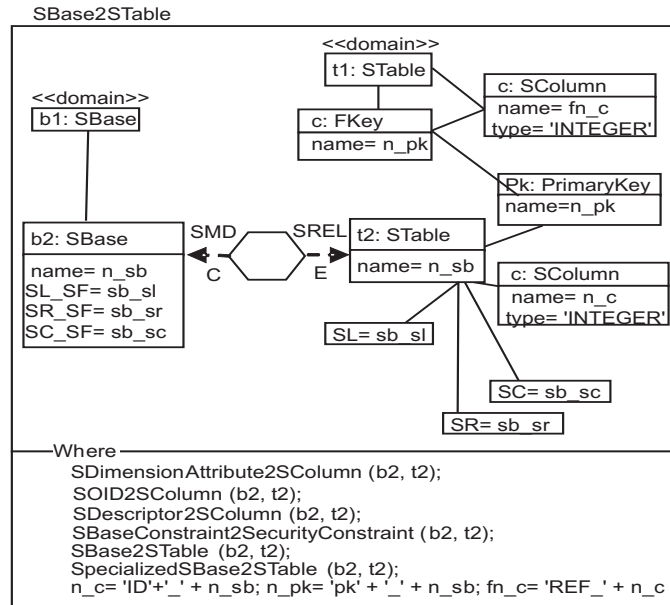
Figure 9: Transforming SBase into STable .
