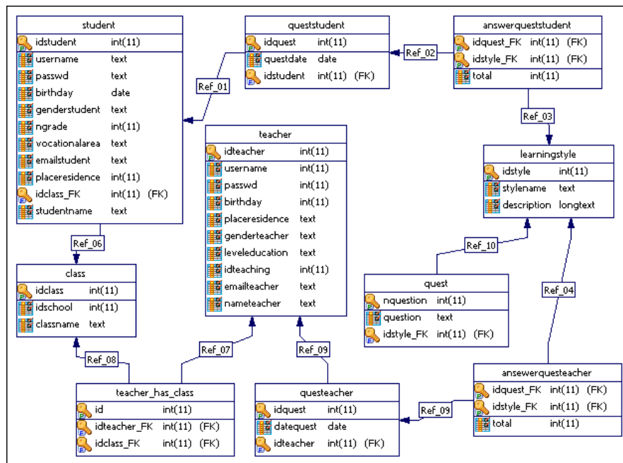
Figure 2: ER Diagram of the MLS database
