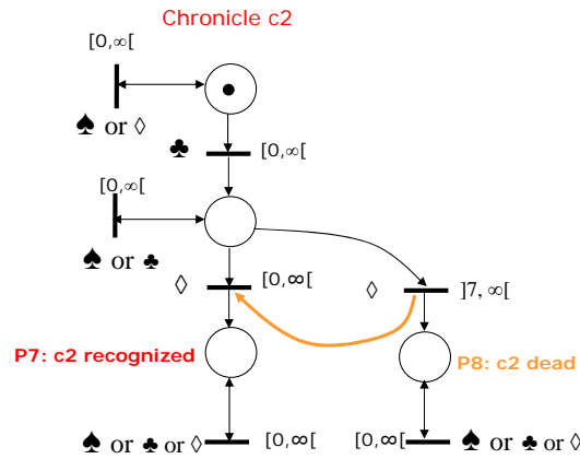
Figure 11: Generator of the chronicle language
