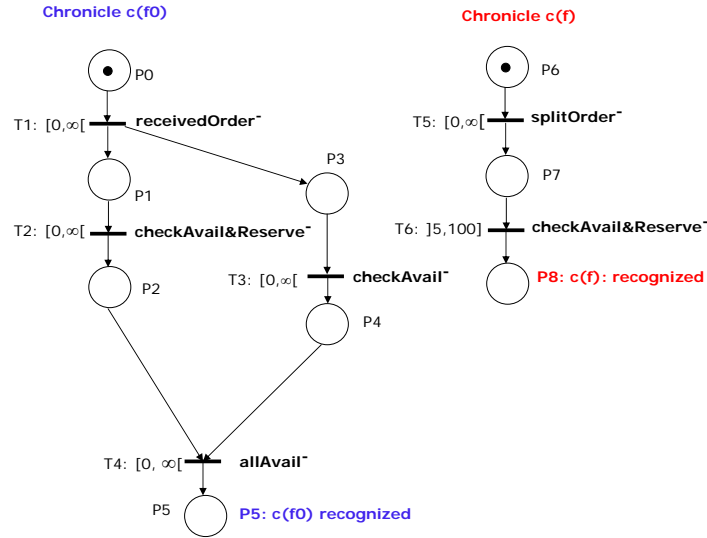
Figure 12: Time Petri Net model for the chronicles of Figure 3
