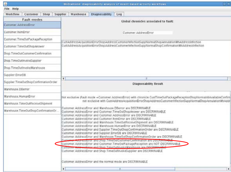
Figure 18: Diagnosability results
