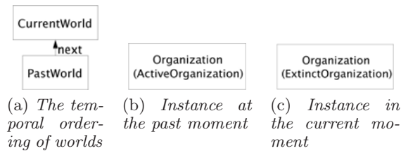
Figure 4: Atoms projected by worlds
