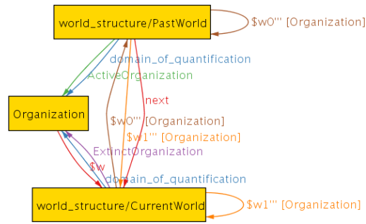
Figure 3: An instance
