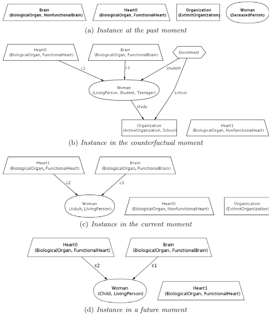
Figure 6: Atoms projected by worlds
