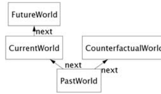
Figure 5: The temporal ordering of worlds
