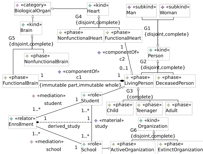
Figure 2: Running example
