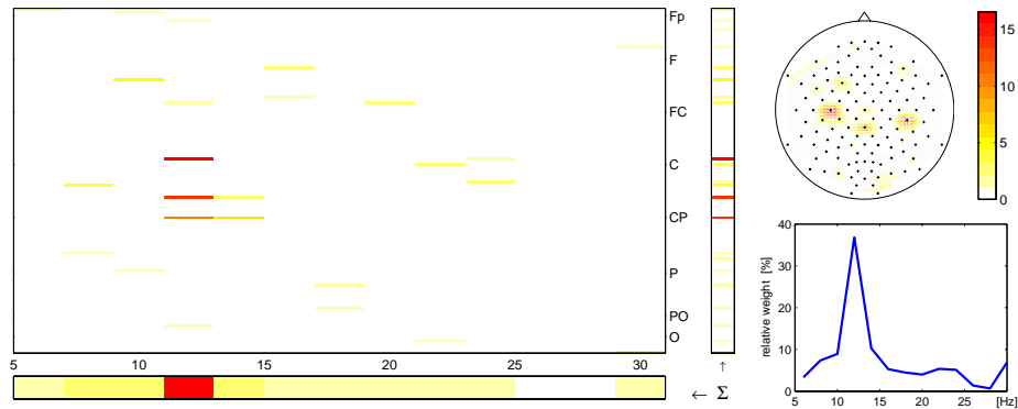
Figure 13: This figure shows the weight vector (display as a channel \times frequency matrix) of a sparse classifier (absolute values) that was trained to discriminate left vs right hand motor imagery. The bar on the bottom shows the sum across all channels and is displayed also in the lower right plot. The focus in the frequency range lies on the \alpha -band (here 11–14 Hz). The bar on the right side of the matrix show the sum across all frequency bands and is displayed as scalp topography in the upper right plot. Note that less than 4% of the features were assigned non-zero weights.
