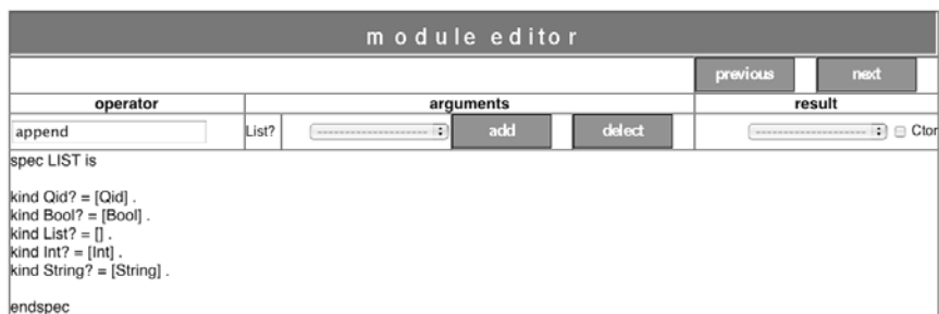
Figure 4: Inserting an operator
