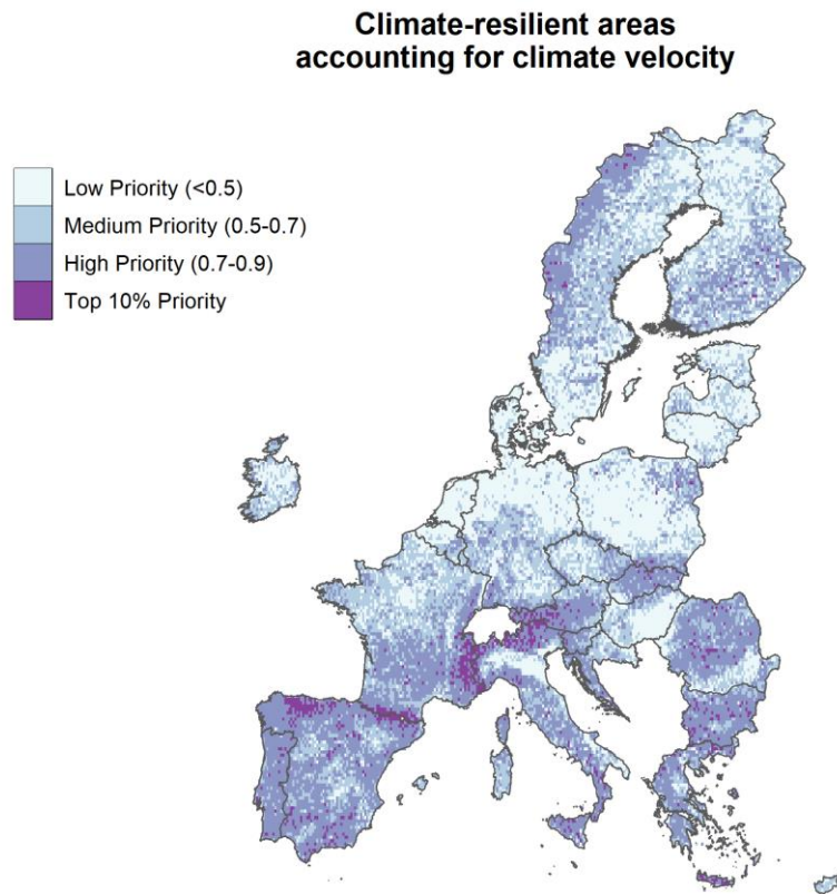
Figure 14: Priority ranking for EU Member States based on the optimal prioritisation weighting scheme, incorporating climate velocity.
