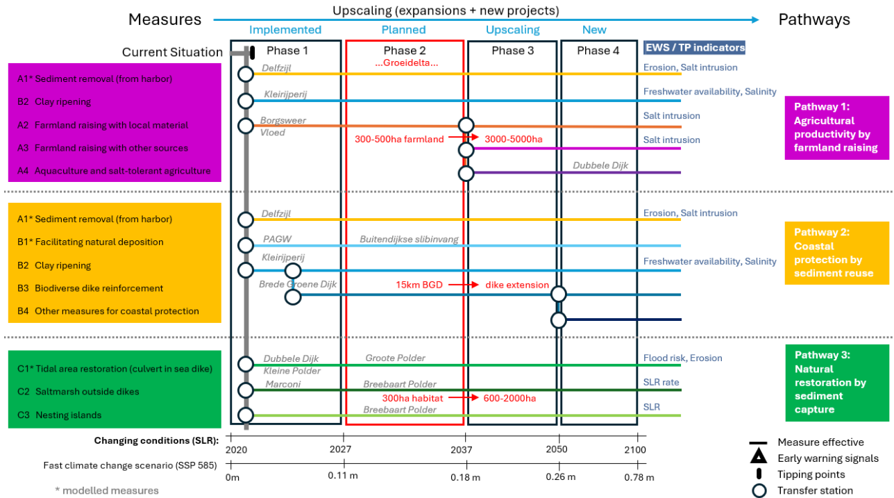
Figure 13: The adaptation pathway map of Ems-Dollard, with a condition-based scenario of SLR
