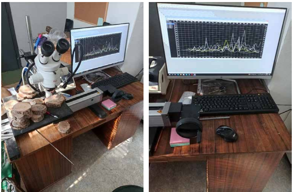
Figure 2. LINTAB 5 tree-ring measurement equipment
