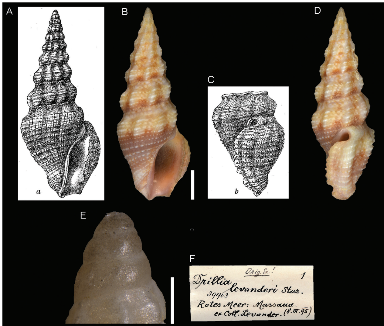
Figure 1. Drillia levanderi Sturany, 1905, Massaua, Eritrea. A, C. Original figures in Sturany, 1905; B, D, E. Holotype NHMW-Mollusca 39903: front ( B ), side ( D ), apex detail ( E ); F. Original label. Scale bars: B, D: 3 mm, E: 0.5 mm.
