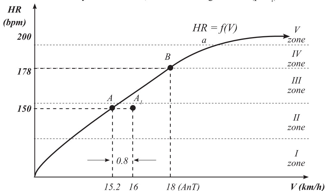
Figure 2. Graph model of the modelled running index (RI)
