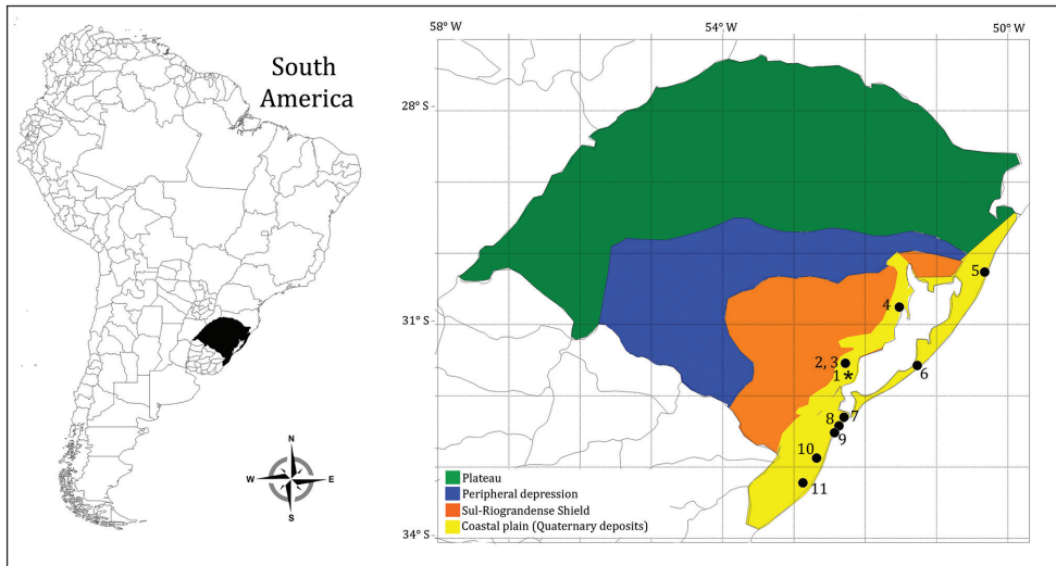
Figure 1. Four main geological formations from the state of Rio Grande do Sul, Southern Brazil. The study area (Quaternary deposits) as well as previous studies used in Dice Similarity Index analysis is entirely inserted in Coastal Plain. Key: 1 present study 2 Turuçu River basin; Burns et al. 2015 3 Corrientes Stream; Volcan et al. 2012 4 Tapes Butiazais ; Becker et al. 2007 5 Fortaleza lagoon; Schifino et al. 2004 6 Lagoa do Peixe; Loebmann and Vieira 2005 7 Peat forest; Quintela et al. 2007 8 Rio Grande coastal streams; Tagliani 1995 9 Cassino coastal streams; Bastos et al. 2013 10 Taim wetland; Garcia et al. 2006 11 Lagoa Mangueira; Artioli et al. 2009.
