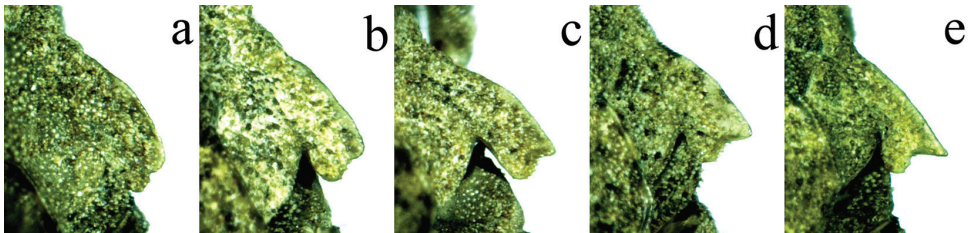
Figure 3. Outline of lateral lobes of pronotum with apex of posterior angle of different individuals of Thoradonta varispina sp. n..
