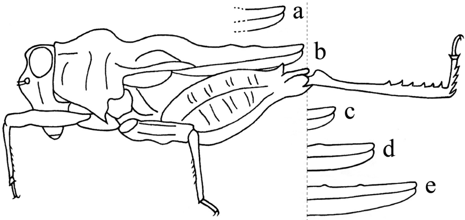
Figure 6. Variations of the length of pronotum in the genus Thoradonta : a hind process of pronotum doesn't reach apex of hind femur b reaches apex of hind femur c slightly surpasses apex of hind femur d nearly reaches middle of hind tibia e nearly reaches apex of hind tibia.
