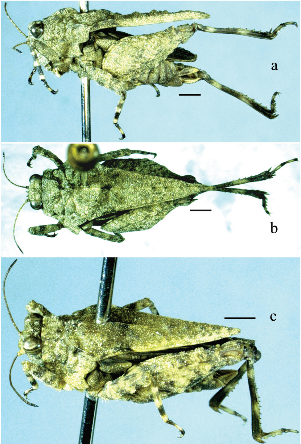
Figure 1. Thoradonta varispina sp. n.: a–b lateral and dorsal views of female c oblique view of male. Scale bars: 1.0 mm.
