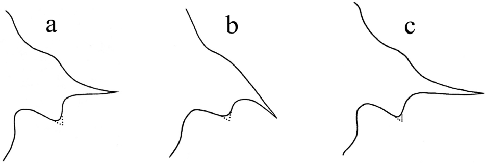
Figure 5. Variations of spine of posterior angle of lateral lobe of pronotum in the genus Thoradonta : a normal and pointing laterally b normal and oblique backward c long and pointing laterally.
