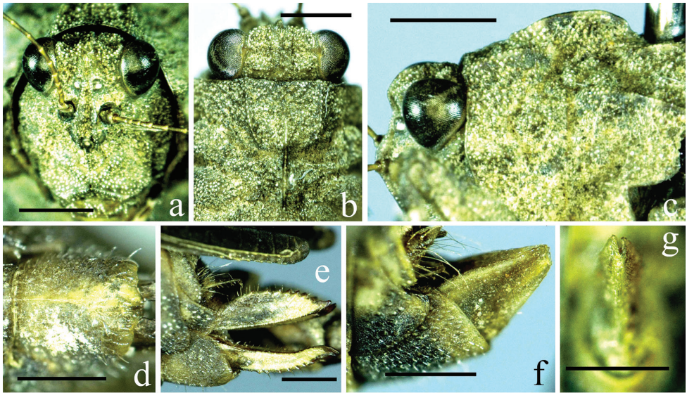
Figure 2. Thoradonta varispina sp. n.: a frontal view of female head b dorsal view of female head and anterior part of pronotum c lateral view of female head and anterior area of pronotum d ventral view of female subgenital plate e lateral view of female ovipositor f lateral view of male subgenital plate g posterior view of male subgenital plate. Scale bars a–c : 1.0 mm, d–g : 0.5 mm.
