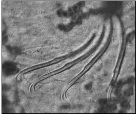
Figure 8. Multiple bifid ventral chaetae.
