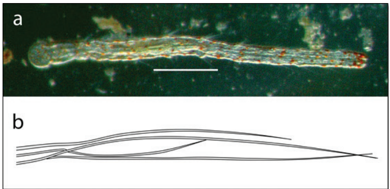
Figure 16. Aeolosoma cf. quarternarium : A photo of entire body showing red epidermal glands and disc-like anterior (scale 200 μm) B typical variable bundle of chaetae.
