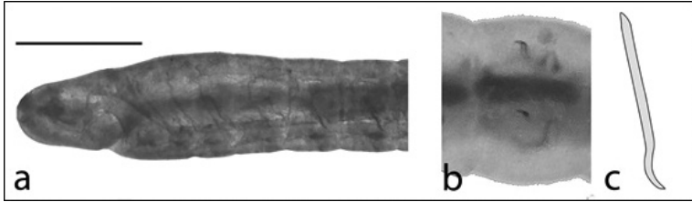
Figure 4. Haplotaxis cf. gordioides : A lateral view of anterior end showing prostomium and ventral mouth (scale 750 μm) B ventral view of one segment showing the two single ventral chaetae C drawing of one ventral chaeta.
