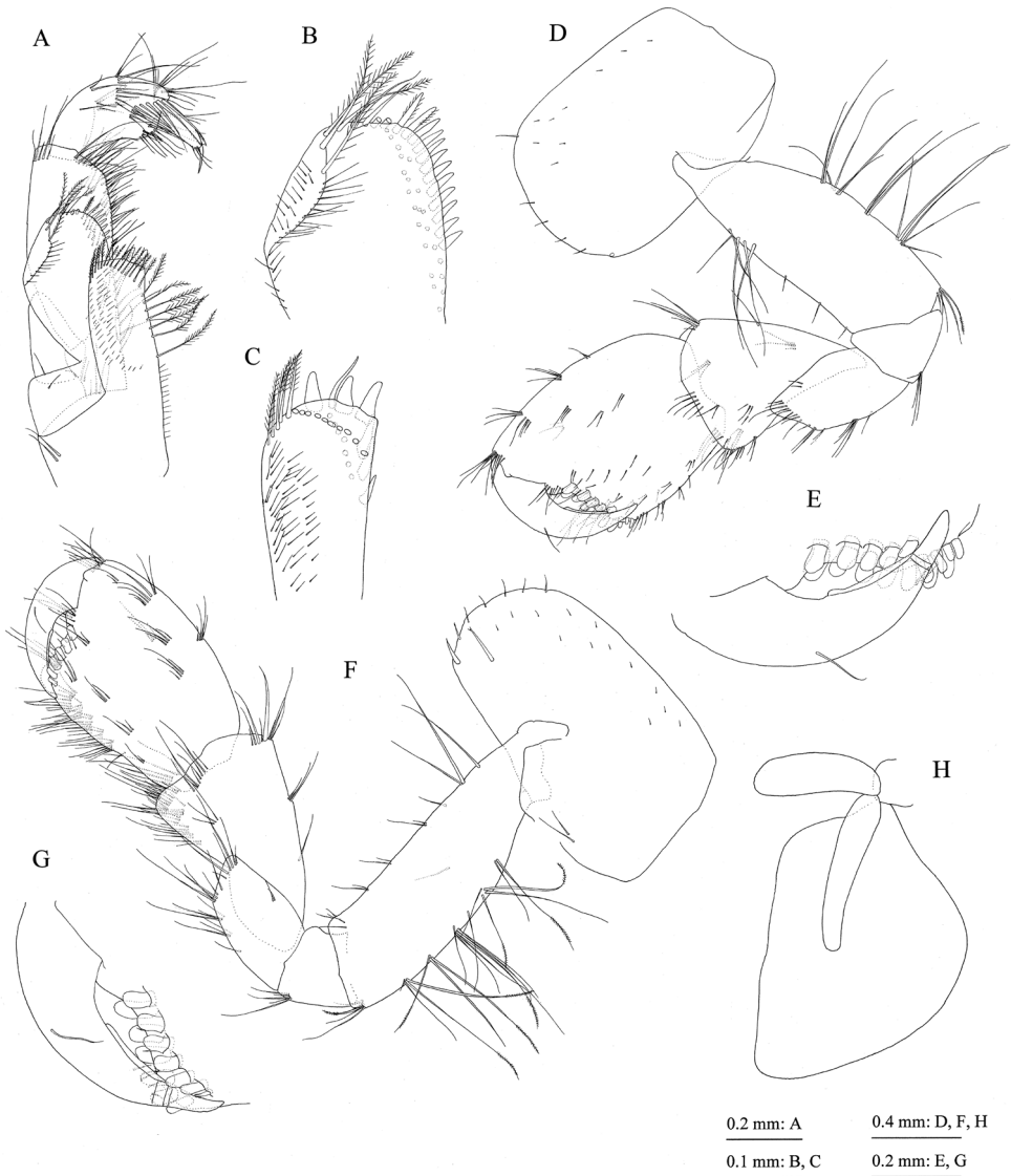
Figure 6. Jesogammarus (Jesogammarus) ikiensis sp. n., holotype, male, 13.1 mm, NSMT-Cr 24107, Ishida, Iki, Nagasaki Prefecture, Japan. A maxilliped, dorsal view B outer plate of maxilliped, dorsal view C inner plate of maxilliped, dorsal view D gnathopod 1, medial view E palmar margin of propodus and dactylus of gnathopod 1, medial view F gnathopod 2, medial view G palmar margin of propodus and dactylus of gnathopod 2, medial view H coxal gill of gnathopod 2, medial view.
