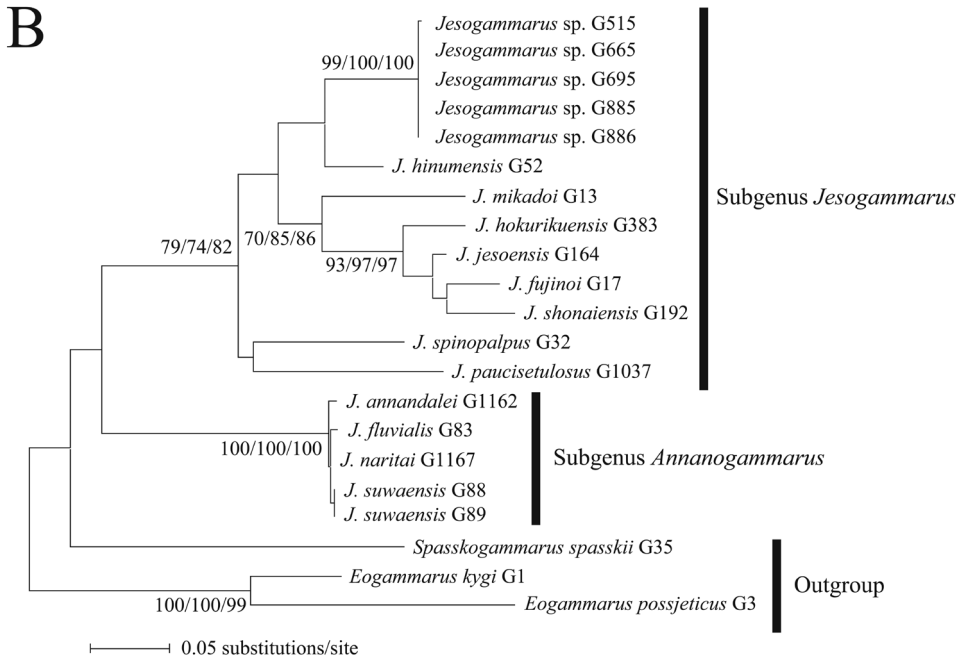
Figure 2. A maximum-likelihood tree from a 333 bp sequence of COI gene B maximum-likelihood tree from a 416 bp sequence of 16S rRNA gene. Numbers near the branches are ML/NJ/MP bootstrap values. Bootstraps are shown when \geq 70\% . Vouchers are shown after species names as in Table 1.
