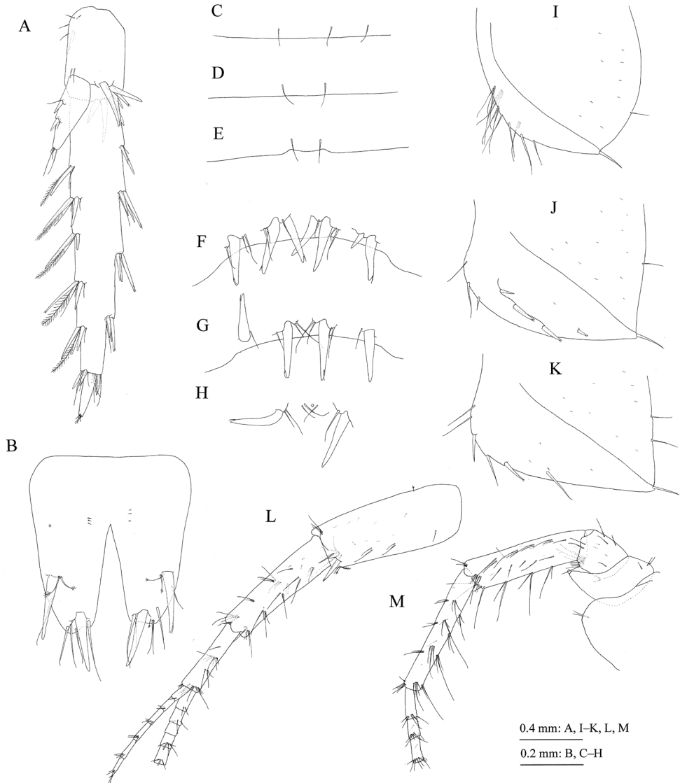
Figure 9. Jesogammarus (Jesogammarus) ikiensis sp. n., Ishida, Iki, Nagasaki Prefecture, Japan. Holotype, male, 13.1 mm, NSMT-Cr 24107 (A–K) and paratype, female, 10.4 mm, NSMT-Cr 24108 (L and M). A uropod 3, dorsal view B telson, dorsal view C–E pleonites 1–3, respectively, dorsal views F–H urosomites 1–3, respectively, dorsal views I–K epimeral plates 1–3, respectively, lateral views L peduncular articles 1–3, accessory flagellum, and flagellar articles 1–5 of antenna 1, medial view M peduncular articles 1–5 and flagellar articles 1–3 of antenna 2, medial view.
