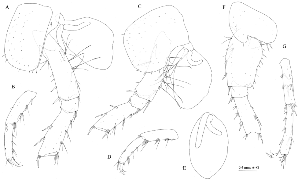
Figure 7. Jesogammarus (Jesogammarus) ikiensis sp. n., holotype, male, 13.1 mm, NSMT-Cr 24107, Ishida, Iki, Nagasaki Prefecture, Japan. A coxa–merus and coxal gill of pereopod 3, lateral view B carpus–dactylus of pereopod 3, lateral view C coxa–merus and coxal gill of pereopod 4, lateral view D carpus–dactylus of pereopod 4, lateral view E coxal gill of pereopod 5, lateral view F coxa–merus of pereopod 5, lateral view G carpus–dactylus of pereopod 5, lateral view.
