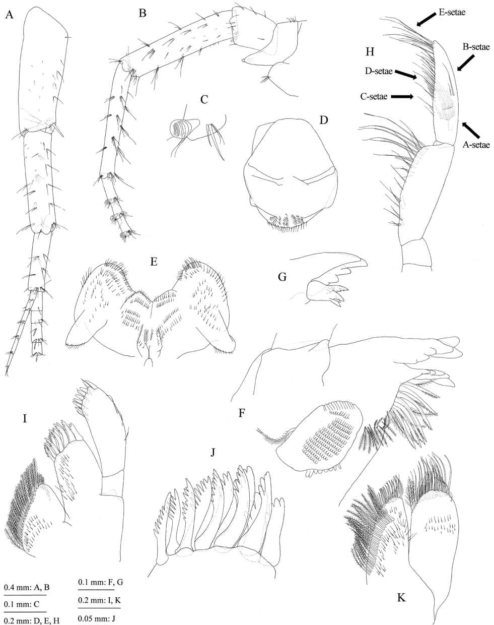
Figure 5. Jesogammarus (Jesogammarus) ikiensis sp. n., holotype, male, 13.1 mm, NSMT-Cr 24107, Ishida, Iki, Nagasaki Prefecture, Japan. A peduncular articles 1–3, accessory flagellum, and flagellar articles 1–4 of antenna 1, medial view (postero-marginal setae on peduncular articles 2 and 3 indicated by arrowheads) B peduncular articles 1–5 and flagellar articles 1–3 of antenna 2, medial view (postero-marginal setae on peduncular articles 4 and 5 indicated by arrowheads) C calceolus of antenna 2, medial view D upper lip, anterior view E lower lip, ventral view F left mandible except palp, medial view G incisor and lacinia mobilis of right mandible, lateral view H palp of right mandible, medial view I maxilla 1, dorsal view J outer plate of maxilla 1, dorsal view K Maxilla 2, dorsal view.
