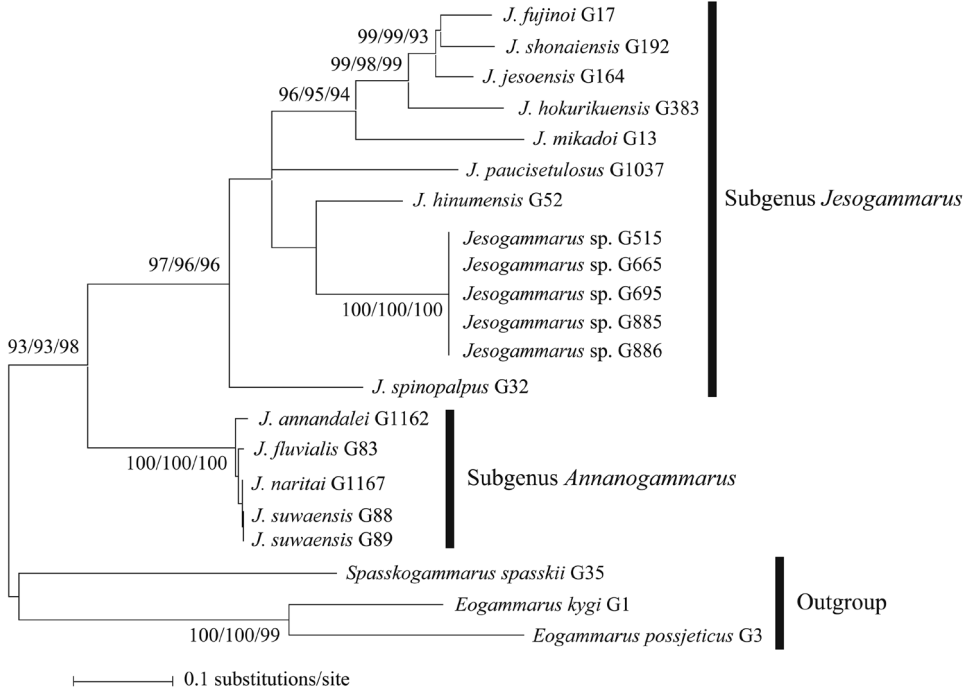
Figure 3. Maximum-likelihood tree from a 749 bp sequence of COI + 16S rRNA genes. Numbers near the branches are ML/NJ/MP bootstrap values. Bootstraps are shown when \geq 70\% . Vouchers are shown after species names as in Table 1.
