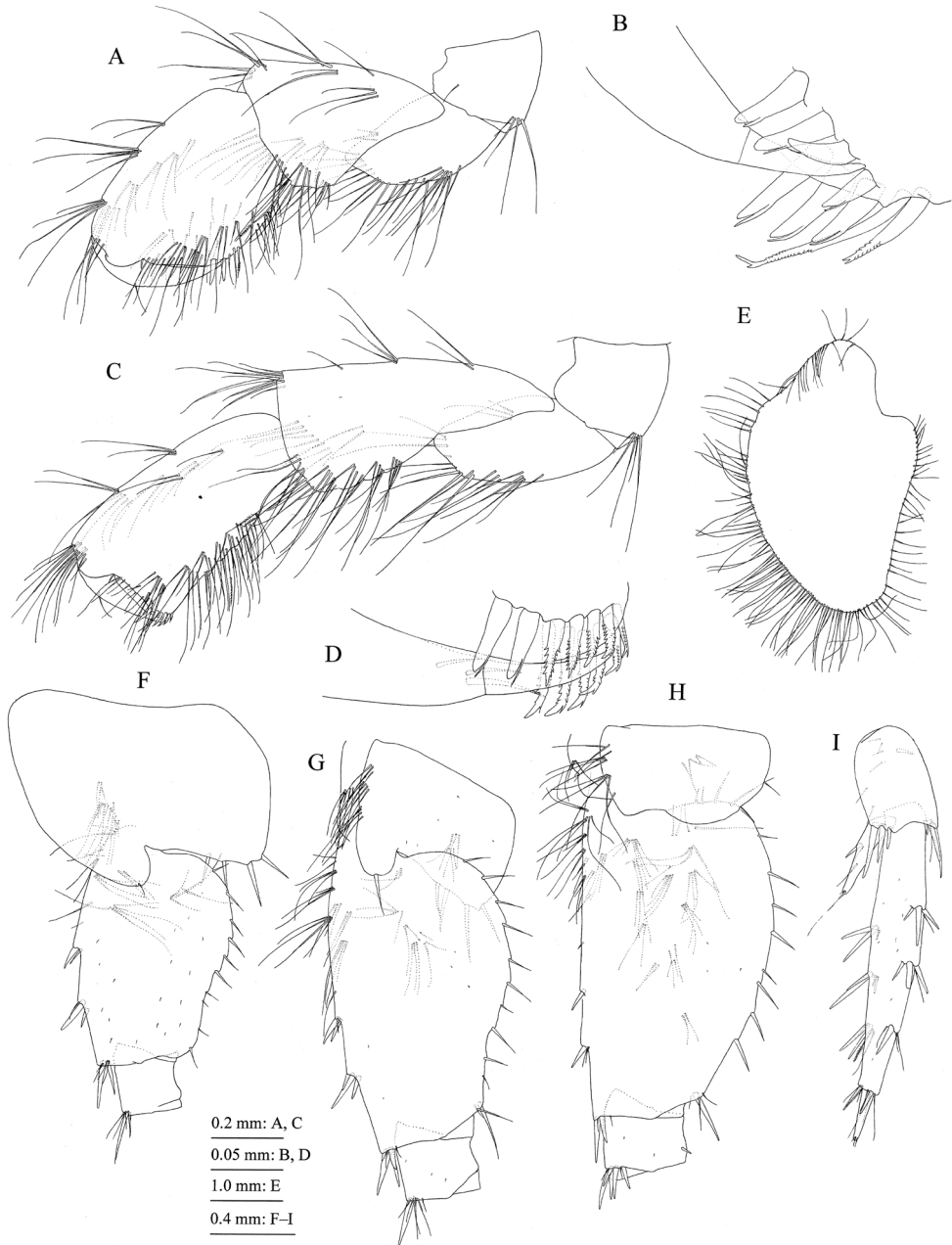
Figure 10. Jesogammarus (Jesogammarus) ikiensis sp. n., paratype, female, 10.4 mm, NSMT-Cr 24108, Ishida, Iki, Nagasaki Prefecture, Japan. A ischium–dactylus of gnathopod 1, lateral view B posterodistal part of palmar margin of propodus and part of dactylus of gnathopod 1, medial view C ischium–dactylus of gnathopod 2, lateral view D posterodistal part of palmar margin of propodus and part of dactylus of gnathopod 2, medial view E brood plate of gnathopod 2, lateral view F coxa–ischium of pereopod 5, lateral view G coxa–ischium of pereopod 6, lateral view H coxa–ischium of pereopod 7, lateral view I uropod 3, ventral view.
