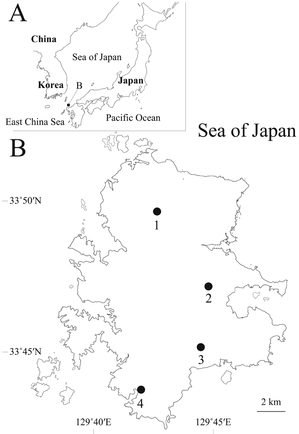
Figure 1. Sampling localities for Jesogammarus (Jesogammarus) ikiensis sp. n. A Map of Japan and adjacent area showing Iki Island, Nagasaki Prefecture, Japan B the collecting localities of Iki Island: 1, Katsumoto; 2, Ashibe; 3, Ishida; 4, Gonoura.
