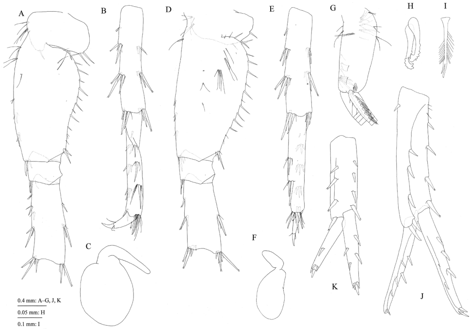
Figure 8. Jesogammarus (Jesogammarus) ikiensis sp. n., holotype, male, 13.1 mm, NSMT-Cr 24107, Ishida, Iki, Nagasaki Prefecture, Japan. A coxa–merus of pereopod 6, lateral view B carpus–dactylus of pereopod 6, lateral view C coxal gill of pereopod 6, lateral view D coxa–merus of pereopod 6, lateral view E carpus–dactylus of pereopod 6, lateral view F coxal gill of pereopod 7, lateral view G pleopod 1, medial view, distal parts of rami omitted H retinacula on peduncle of pleopod 1, medial view I bifid plumose seta (clothes-pin seta) on inner basal margin of inner ramus of pleopod 1, medial view J uropod 1, dorsal view K uropod 2, dorsal view.
