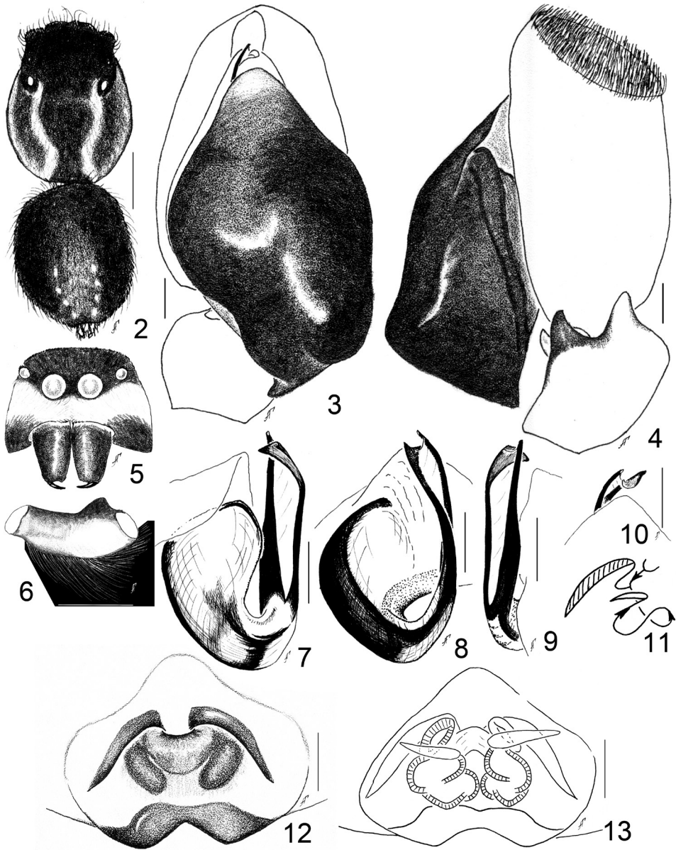
Figures 2–13. Aelurillus albochryseus sp. n.: 2 male, body pattern 3 left palp, ventral view 4 ditto, retrolateral view 5 male face 6 palpal femur, retrolateral view 7 embolic division, retrolateral view 8 ditto, dorsal view 9 ditto, prolateral view 10 ditto, ventral view 11 diagrammatic course of the insemination ducts 12 epigyne, ventral view 13 spermathecae; dorsal view. Scale bars – 0.1 mm ( 3–8, 11–12 ), 0.5 mm ( 10 ), 1 mm ( 2 ).
