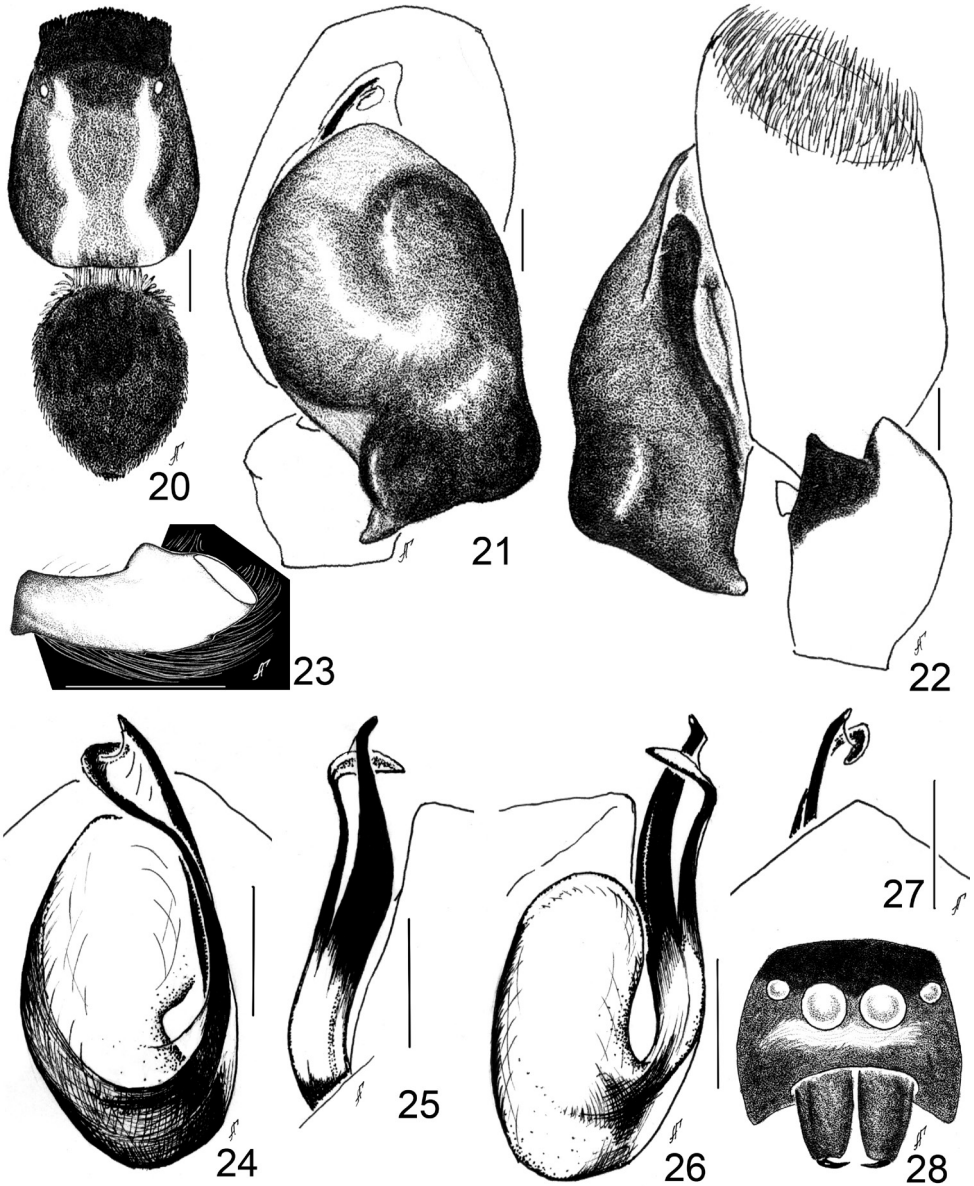
Figures 20–28. Aelurillus deltshevi sp. n.: 20 male, body pattern 21 left palp, ventral view 22 ditto, retrolateral view 23 palp femur, prolateral view 24 embolic division, ventral view 25 ditto, prolateral view 26 ditto, retrolateral view 27 embolic division, ventral view 28 male face; Scale bars – 0.1 mm ( 21–22 , 24–27 ), 0.5 mm ( 23 ); 1 mm ( 20 ).
