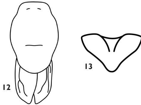
Figures 12–13. Thaumaspis (Thaumaspis) montana Bey-Bienko, 1957 (after Gorochov) 12 pronotum and tegmina, dorsal view 13 subgenital plate of female, ventral view.
