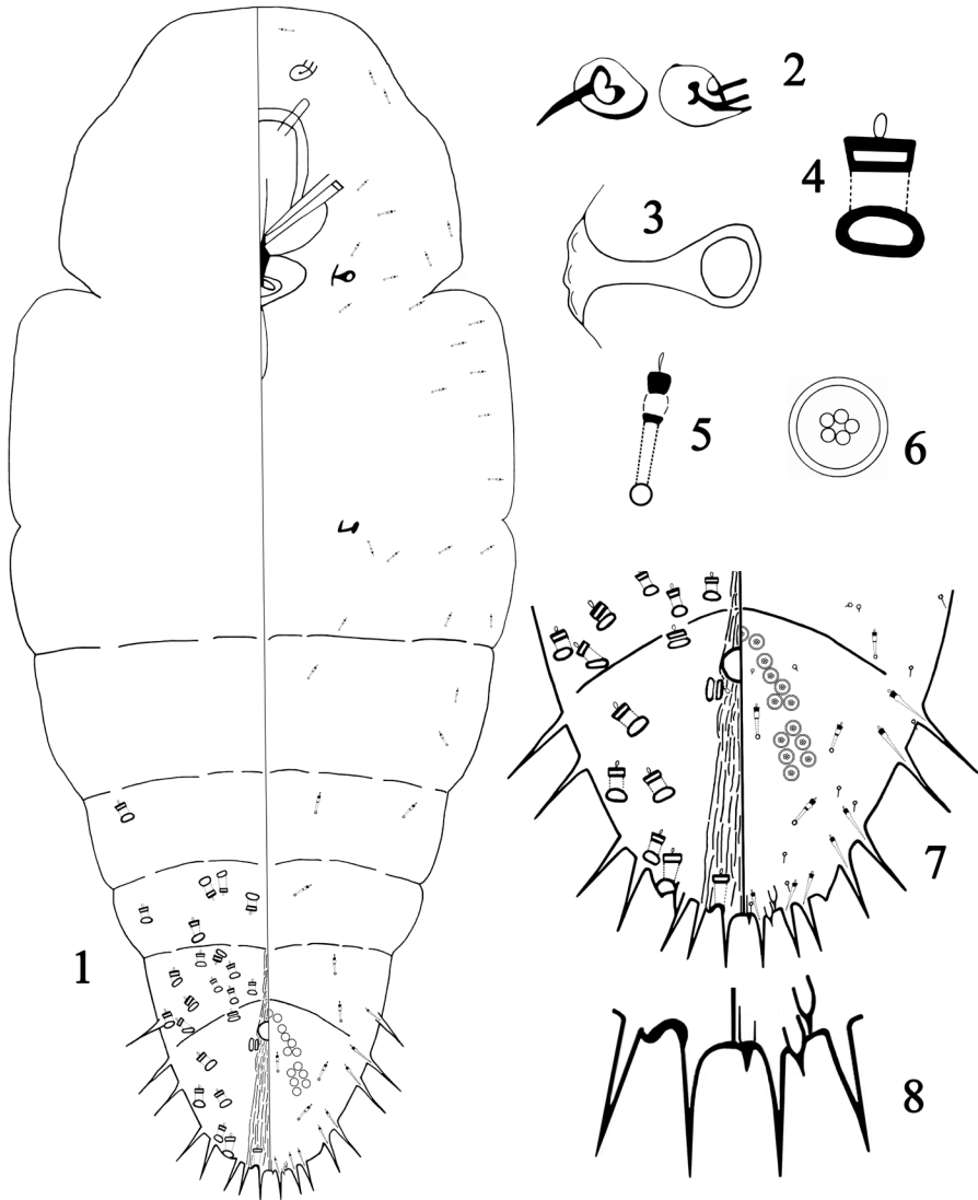
Figures 1–8. Megacanthaspis guiyangensis sp. nov., adult female 1 body 2 antennae 3 anterior spiracle 4 detail of dorsal gland duct 5 ventral microducts 6 perivulvar pore 7 pygidium 8 margin of pygidium (sharp marginal processes).
