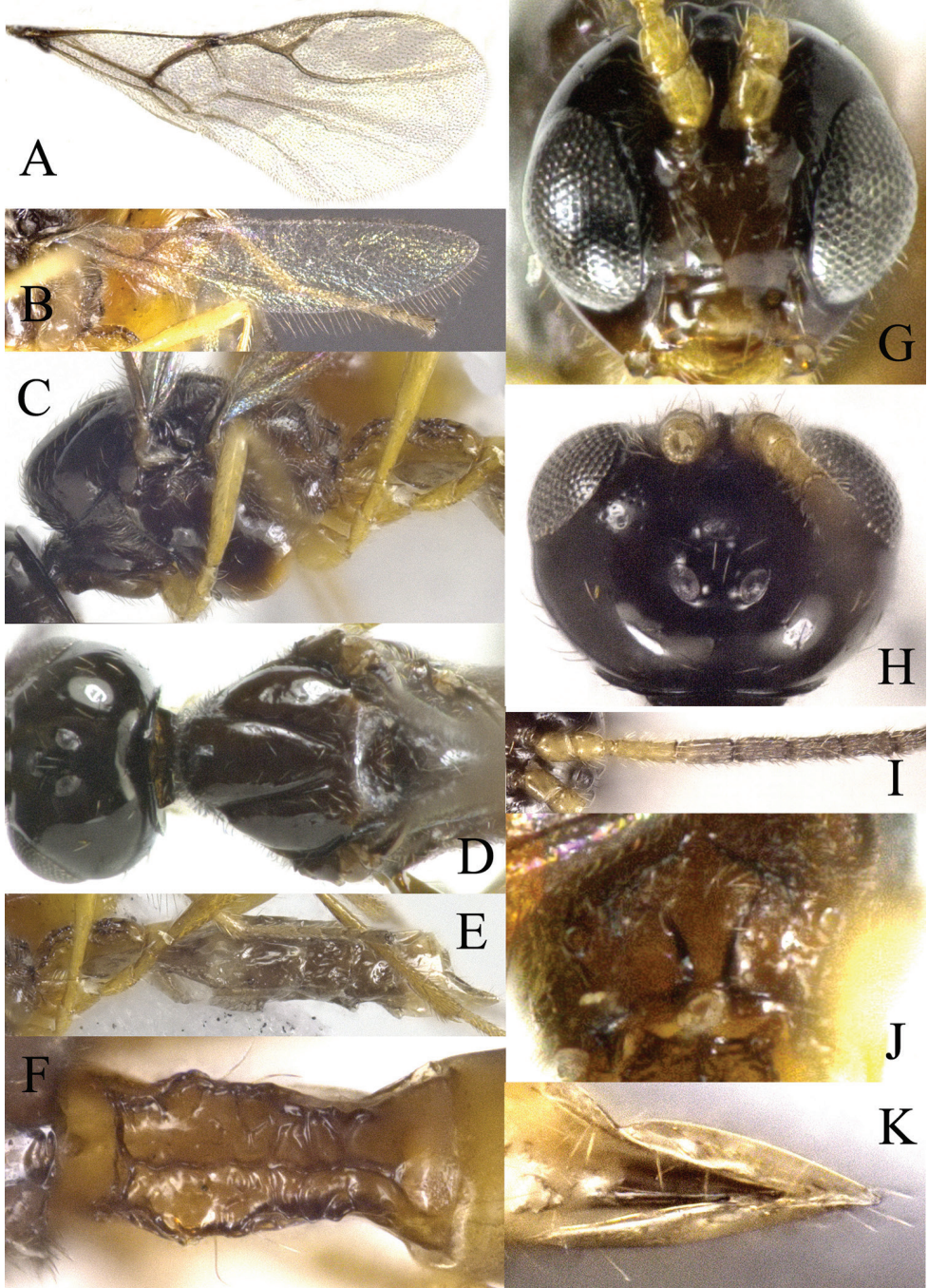
Figure 2. Areopraon chui Tian & Chen, sp. n. A fore wing B hind wing C mesosoma, lateral aspect D mesoscutum, dorsal aspect E metasoma, lateral aspect F T1, dorsal aspect G head, anterior aspect H head, dorsal view I antenna J propodeum, dorsal aspect K ovipositor sheaths, dorsal aspect.
