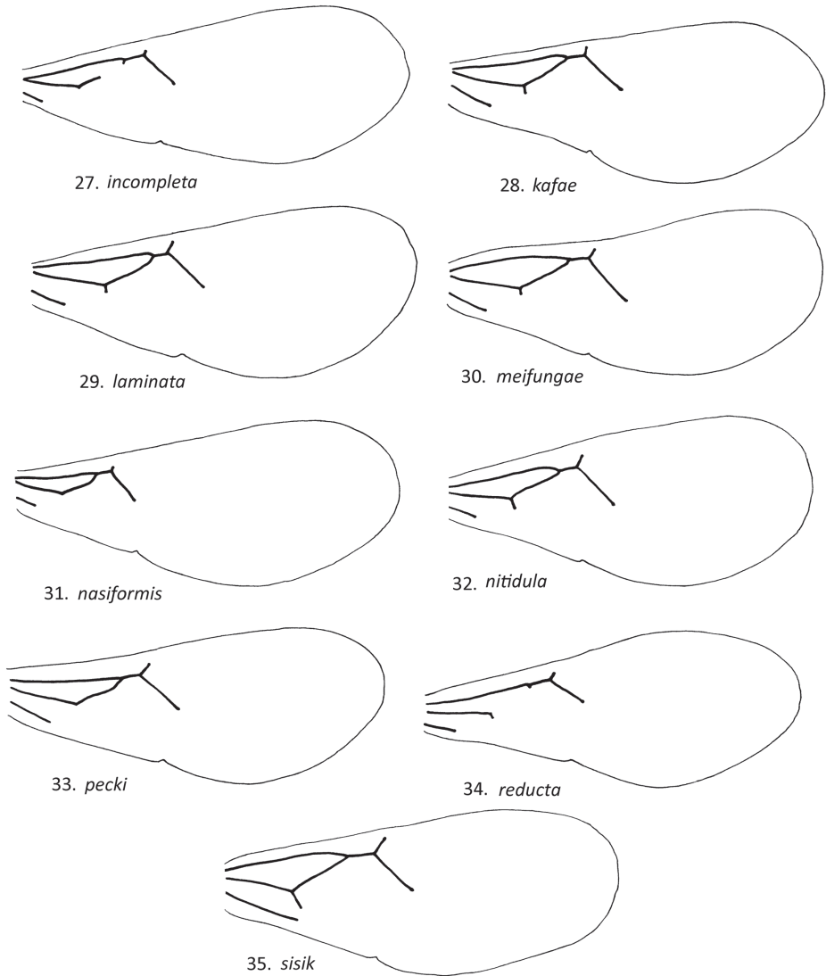
Figures 27–35. Male Loboscelidia forewings.
