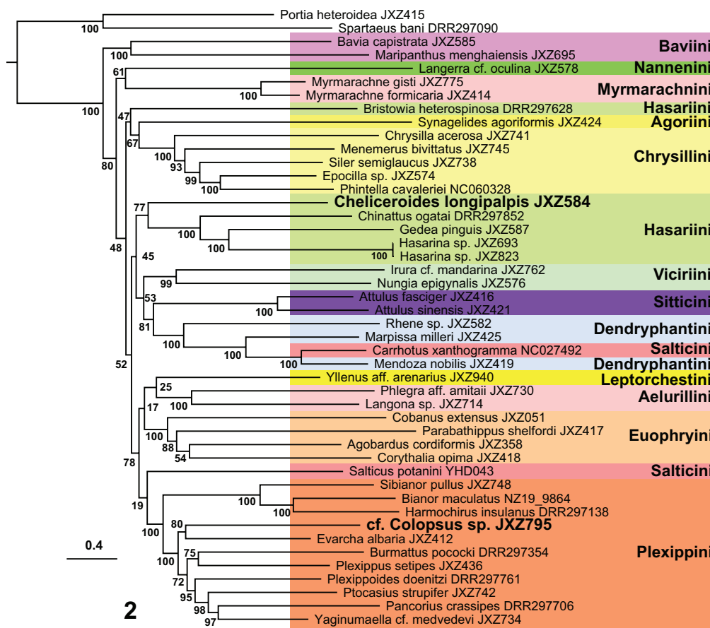
Figures 1, 2. Phylogenetic results 1 maximum-likelihood tree from the UCE dataset 2 maximum-likelihood tree from the 13-mitochondrial-PCG dataset; numbers along the branches indicate bootstrap support.
