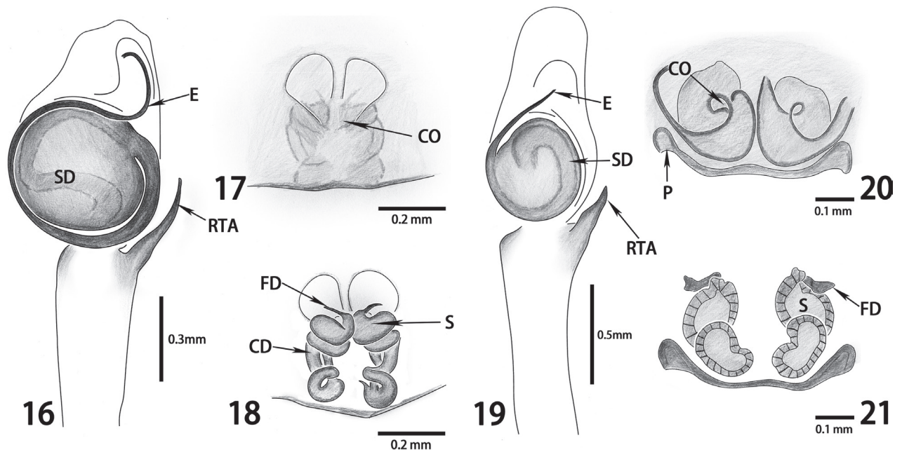
Figures 16–21. Comparison of genital structures of Cheliceroides longipalpis Żabka, 1985 (16–18) and the type species of Colopsus , Colopsus cancellatus Simon, 1902 (19–21, modified from Kanesharatnam and Benjamin 2021) 16, 19 left palp, ventral view 17, 20 epigynum, ventral view 18, 21 epigynum, dorsal view.
