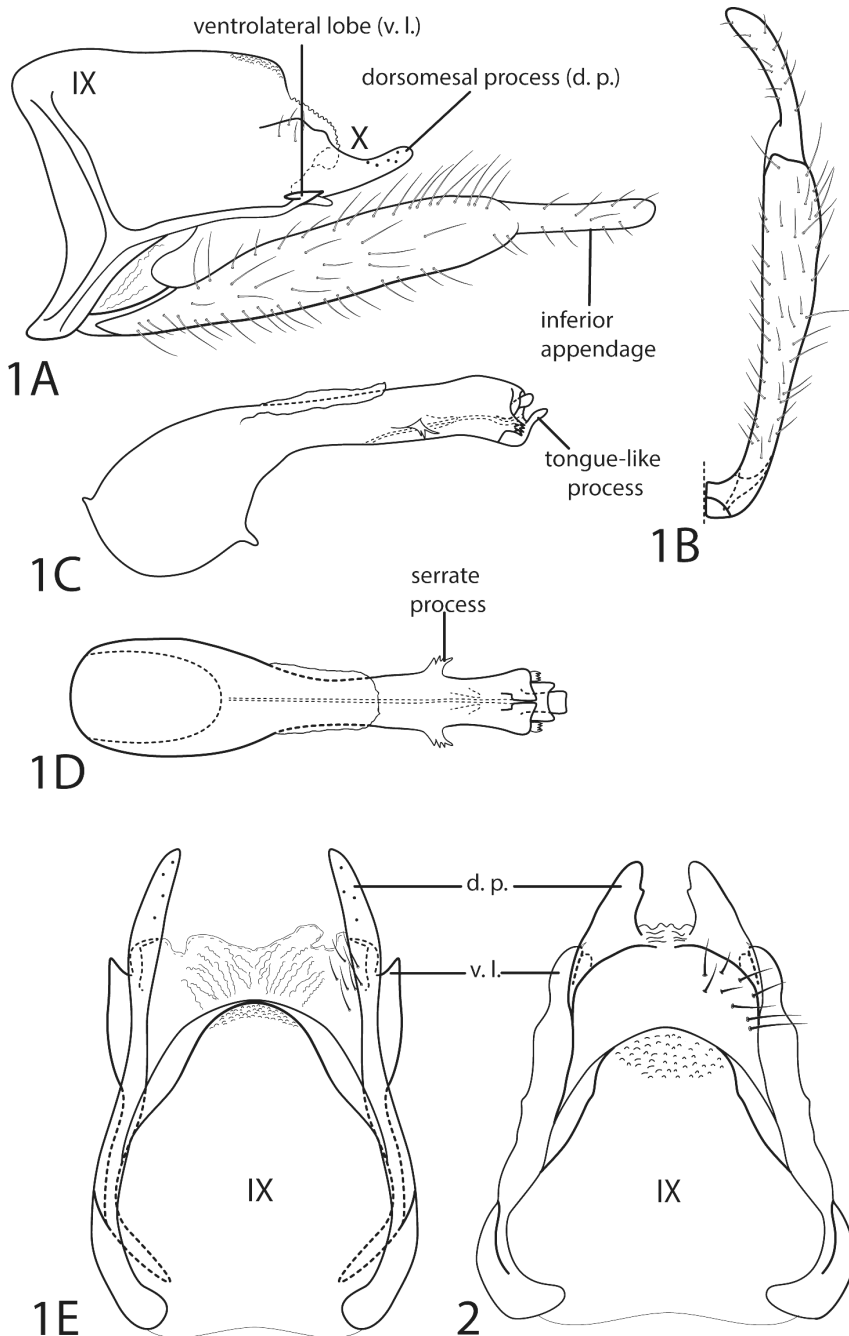
Figure 1–2. Smicridea (R.) lobata (Ulmer, 1909) and Smicridea (R.) signata Banks, 1903, male genitalia. 1A Smicridea (R.) lobata segments IX and X, lateral 1B Left inferior appendage, ventral 1C Phallus, lateral 1D Phallus, dorsal 1E Segments IX and X, dorsal 2 Smicridea (R.) signata . Segments IX and X, dorsal. These illustrations were made from specimens of S. lobata from Zulia and Sucre States, Venezuela, and specimens of S. signata from Utah, USA.
