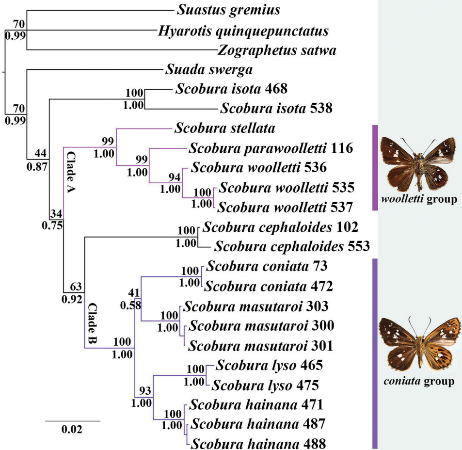
Figure 1. Majority-rule consensus tree from the Bayesian analysis (BI) of the concatenated COI and EF-1 \alpha sequences. Values at nodes represent the bootstrap support (BS) values of the maximum likelihood (ML) and the posterior probabilities (PP) of BI analyses, respectively (BP/PP).
