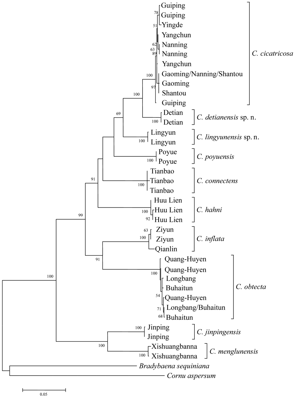
Figure 2. Maximum Likelihood tree based on analysis of the concatenated dataset of COI, 16S, and ITS2 sequences. Numbers beside nodes indicate bootstrapping support (%) for main clades.
