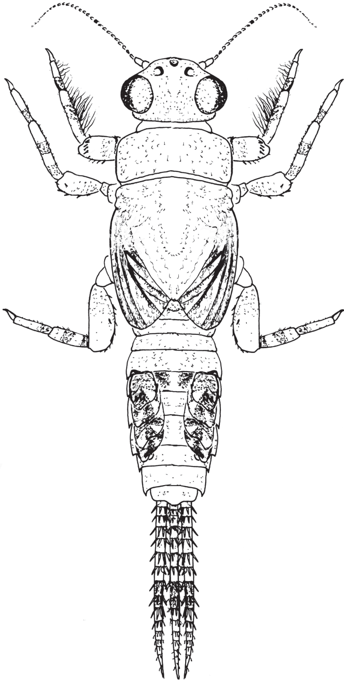
Figure 2. Male nymphal habitus of Teloganopsis setosa sp. n.
