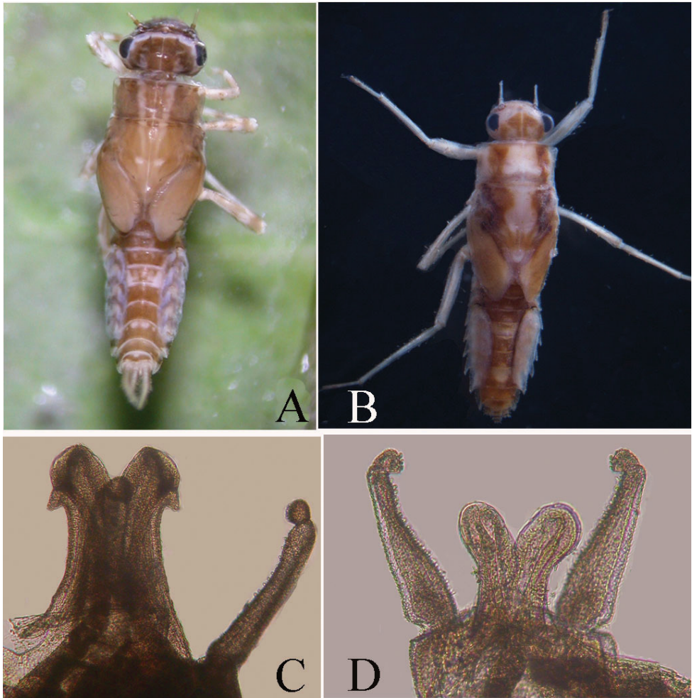
Figure 8. Structures of Teloganopsis punctisetae and T. jinghongensis (digital photographs) A T. punctisetae nymph (dorsal view) B T. jinghongensis nymph (dorsal view) C T. punctisetae genitalia (ventral view) D T. jinghongensis genitalia (ventral view).
