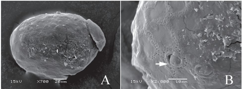
Figure 7. Teloganopsis setosa sp. n. Egg morphology (SEM photos) A whole egg B egg surface enlarged (arrow indicates the projection).
