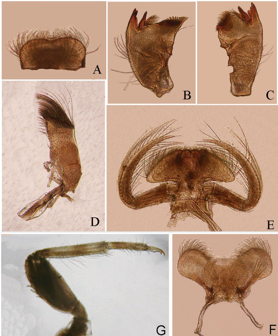
Figure 3. Structures of Teloganopsis setosa sp. n. nymph (digital photographs) A labrum (dorsal view) B right mandible C left mandible D maxilla E labium (ventral view) F hypopharynx (dorsal view) G foreleg.
