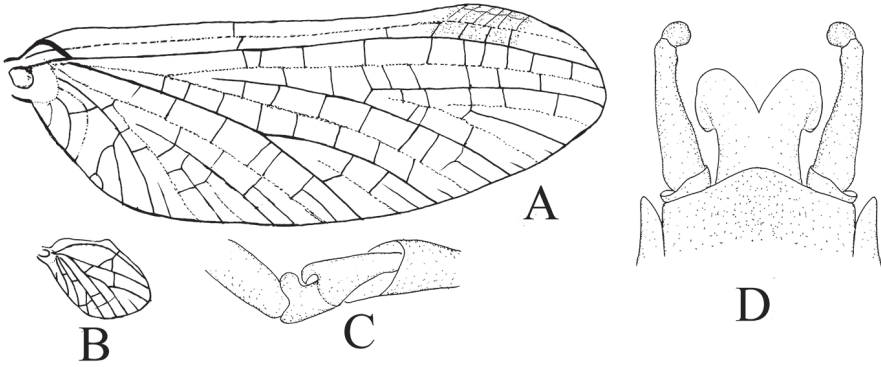
Figure 6. Male structures of Teloganopsis setosa sp. n. A forewing B hindwing C joint of tarsi and tibiae of foreleg D genitalia (ventral view).
