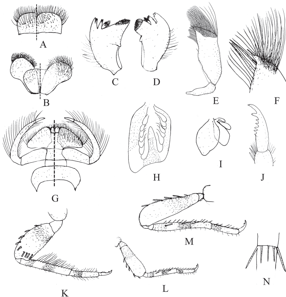
Figure 4. Nymphal characters of Teloganopsis setosa sp. n. A labrum (dorsal view on left; ventral view on right) B hypopharynx (dorsal view on left; ventral view on right) C right mandible D left mandible E maxilla F apex of maxilla G labium (dorsal view on left; ventral view on right) H gill I (ventral view) I gill V (dorsal view) J claw K foreleg L midleg M hindleg N articulation of caudal filaments.
