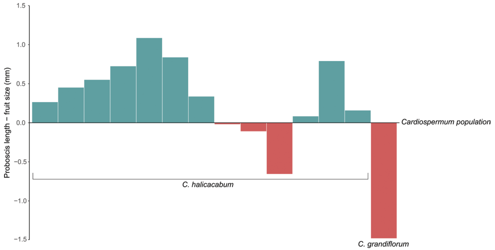
Figure 6. Difference between average proboscis length and average fruit size (i.e. proboscis length - fruit size) for Leptocoris mutilatus and Cardiospermum populations in KNP. Green bars represent populations in which soapberry bugs are well-suited to feed on their Cardiospermum hosts (i.e. proboscis length > fruit size) and red bars represent populations in which soapberry bugs are poorly matched (i.e. proboscis length < fruit size).
