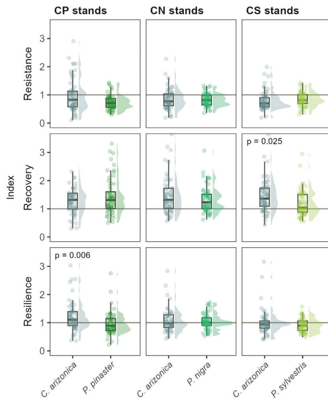
Figure 2. Boxplots of growth resistance, recovery and resilience indices to drought events over the period 1974–2018 for each mixed forest type and species. P-values show significant differences between species. Ca: Cupressus arizonica ; Pp: Pinus pinaster ; Pn: Pinus nigra ; Ps: Pinus sylvestris . CP: Cupressus arizonica and Pinus pinaster mixed stands; CN: C. arizonica and P. nigra mixed stands; CS: C. arizonica and P. sylvestris mixed stands.
