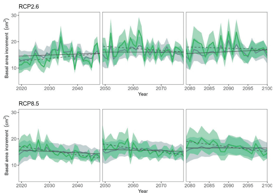
Figure 4. Mean predicted basal area increment (BAI) ( \pm 95% confidence interval) over the projected period (2019–2100) for C. arizonica (grey) and P. nigra (green) mixed forest under forcing scenarios RCP2.6 and RCP8.5. Solid and dashed black lines represent growth trends for C. arizonica and P. nigra , respectively.
