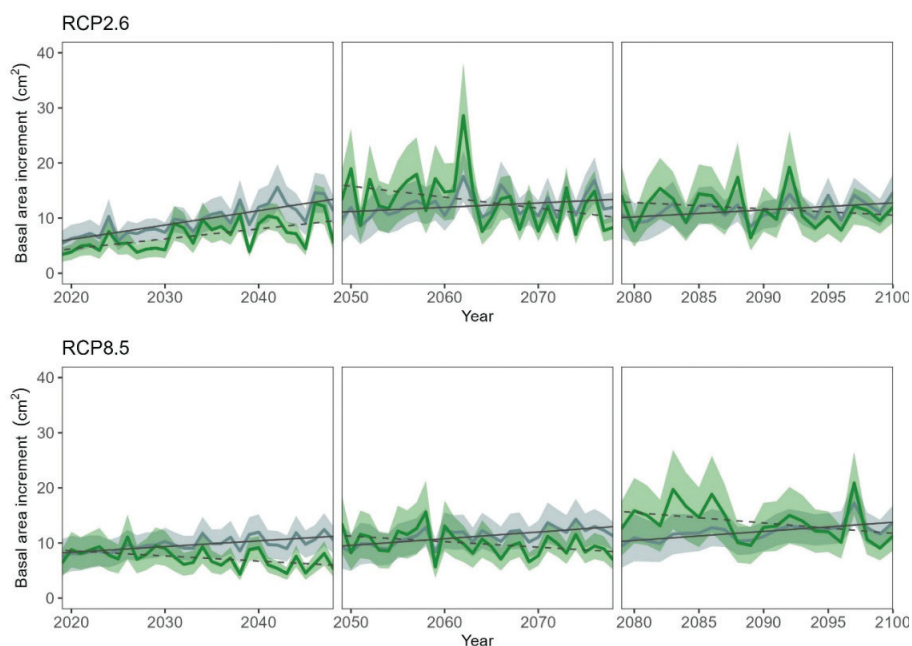
Figure 3. Mean predicted basal area increment (BAI) ( \pm 95% confidence interval) over the projected period (2019–2100) for C. arizonica (grey) and P. pinaster (green) mixed forest under forcing scenarios RCP2.6 and RCP8.5. Solid and dashed black lines represent growth trends for C. arizonica and P. pinaster , respectively.
