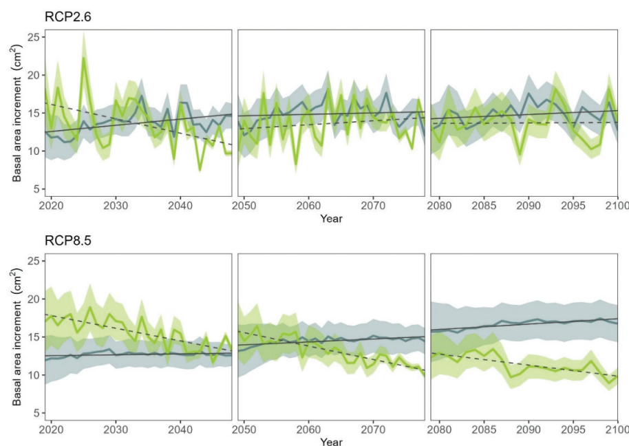
Figure 5. Mean predicted basal area increment (BAI) ( \pm 95% confidence interval) over the projected period (2019–2100) for C. arizonica (grey) and P. sylvestris (green) mixed forest under forcing scenarios RCP2.6 and RCP8.5. Solid and dashed black lines represent growth trends for C. arizonica and P. sylvestris , respectively.
