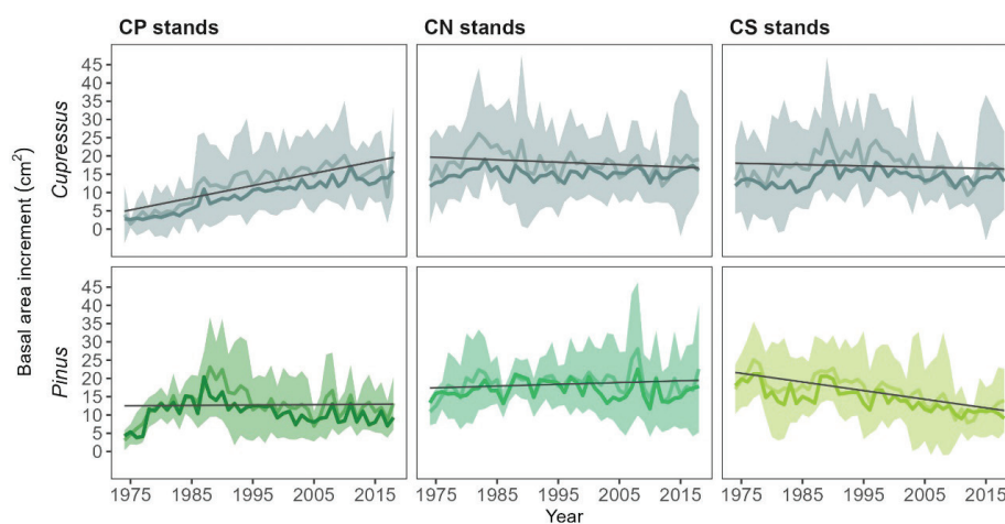
Figure 1. Mean observed ( \pm SD; light colours) and predicted basal area increment (dark colours) over the period 1974–2018 for each mixed forest type and species. Black lines represent growth trends for the study period. CP: Cupressus arizonica and Pinus pinaster mixed stands; CN: C. arizonica and P. nigra mixed stands; CS: C. arizonica and P. sylvestris mixed stands.
