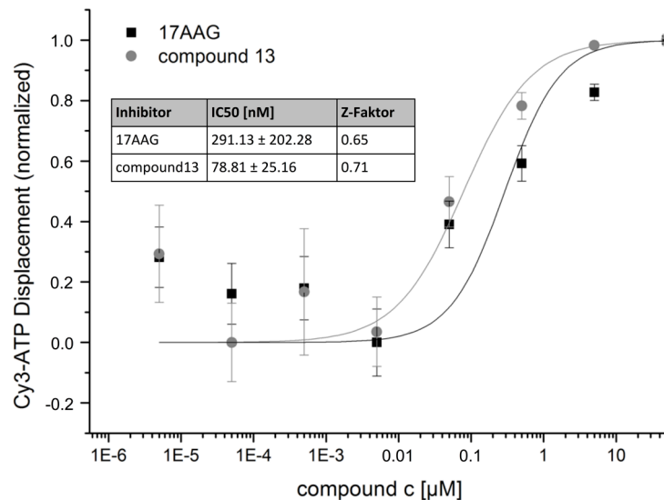
Figure 2a. Typical displacement assay of Cy3-ATP on AtHSP83 by geldanamycin derivative. Purified AtHSP83 was printed on the microarray surface and Cy3-ATP was competed by a geldanamycin derivative, synthesis and properties given in Schax et al., [13]. The IC_{50} value was obtained from dose-response curve fittings.
