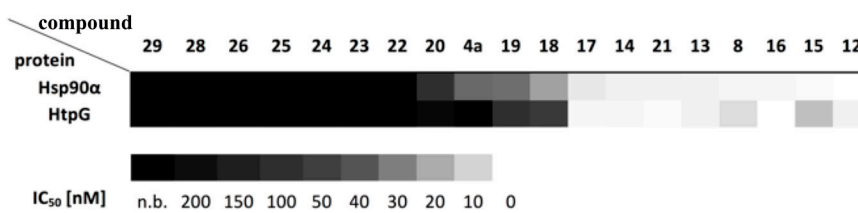
Figure 2b. Heat map of the calculated IC_{50} values of HSP90 \alpha from H. sapiens , HtpG from H. pylori and HSP83 from A. thaliana for several tested potential inhibitors in a competitive displacement assay. Numbers as indicated have been described before [13]. Different grey tones from black to white indicate the potency of the inhibitor. White corresponds strong inhibitory effects, whereas black shows no effects for the competition with ATP for the binding pocket.
