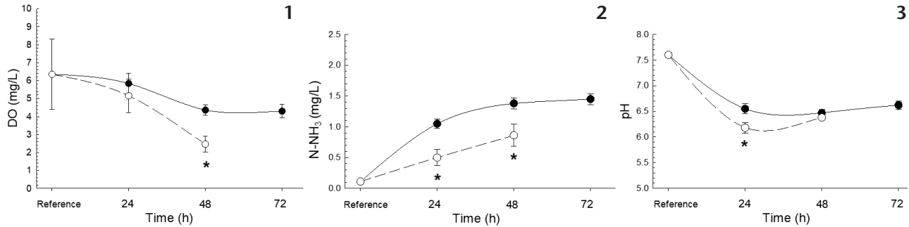
Figures 1–3. Time course of variation of water parameters for living and dead A. saxatilis : (1) water dissolved oxygen (DO, mg/L), (2) total ammonia-N ( \text{NH}_3\text{-N} , mg/L) and (3) pH versus time (h). Values shown are means \pm SEMs. When not apparent, SEM is smaller than the symbol. This happened for the water of the reference fish, ammonia and pH. Black circles: fish that were alive at the end of the experiment; white circles: fish that died during the experiment. *: water parameter for dead fish is different from that of live fish.
