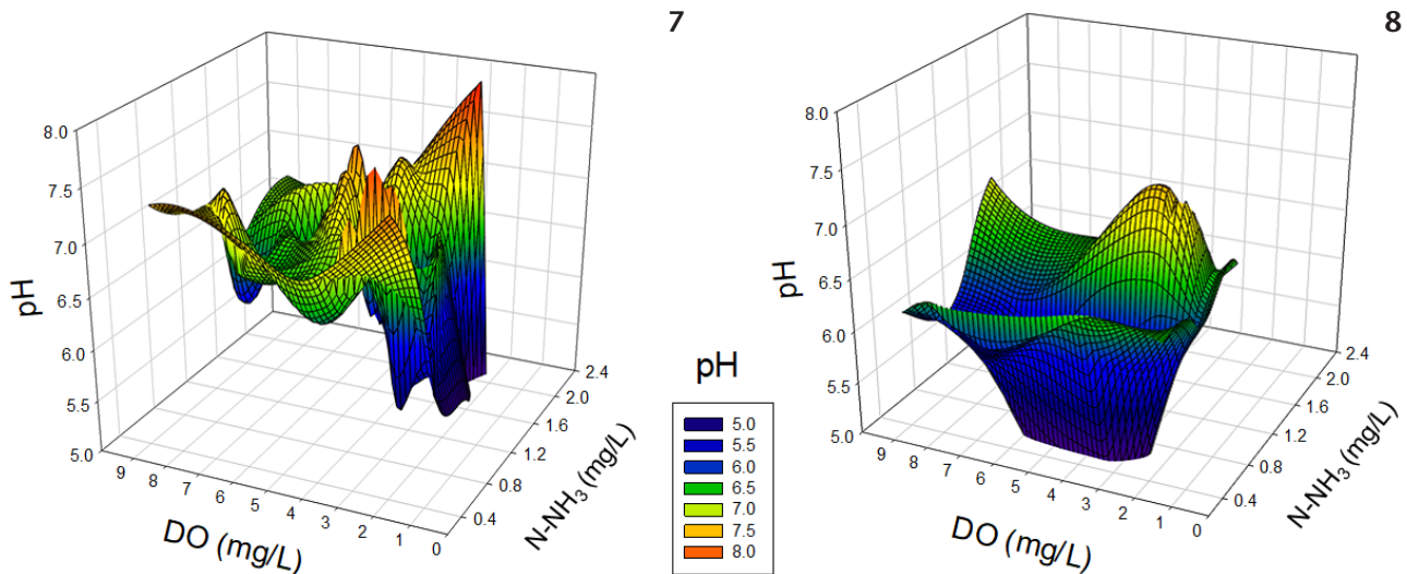
Figures 7–8. 3-D mesh plots showing the relationship among the 3 water parameters, whole set of data. \text{NH}_3\text{-N} (mg/L) versus DO(mg/L) versus pH, for live (7) and dead (8) fish. Legend illustrates color codes for pH interpolation.
