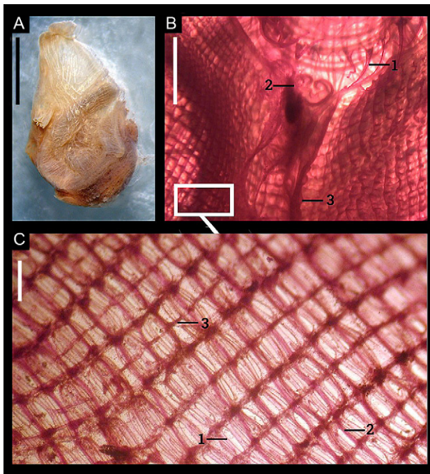
Figure 2. Ascidiella scabra (Müller, 1776). A. Specimen (MZUCVI 00003) without tunic from sample PD003-4 from bow-thruster gratings. B. Dissected specimen (MZUCVI 00007) from sample PD003-21 from sea-chest gratings (1 = oral tentacles, 2 = dorsal tubercle, 3 = dorsal lamina). C. Branchial sac detail of the same specimen (1 = stigmata, 2 = longitudinal vessel, 3 = transversal vessel). Scale bars: A = 2 cm; B = 0.5 cm; C = 0.2 cm.
