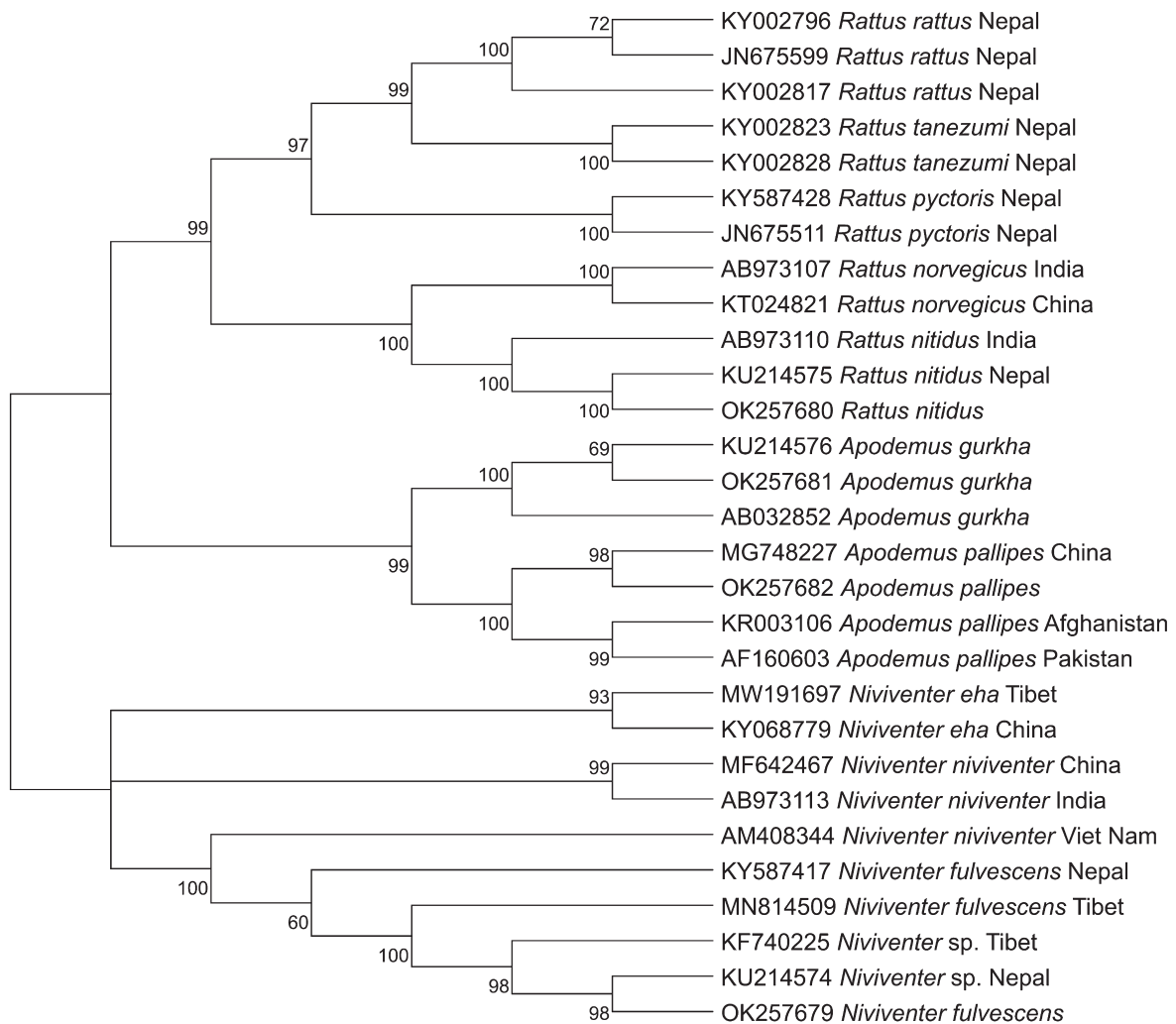
Figure 4. Maximum parsimony tree with bootstrap nodal support of Cytb sequences of representative taxa from Nepal and the surrounding region (Appendix, Table A1) analyzed with the sequences obtained in this study.
