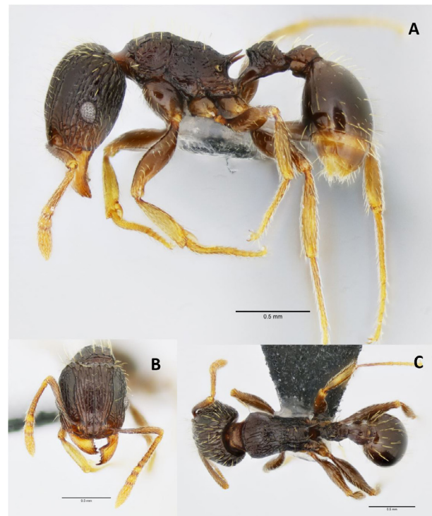
Figure 9. Tetramorium lucayanum (DS086). A. Lateral view B. Frontal view C. Dorsal view. Images by Adrian Troya.
