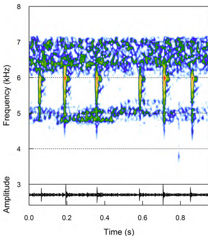
Figure 3. Advertisement call of Pseudopaludicola pocoto recorded in Cabrobó, Pernambuco state, Brazil. Spectrogram (top) and oscillogram (bottom) from two notes (6 pulses).
