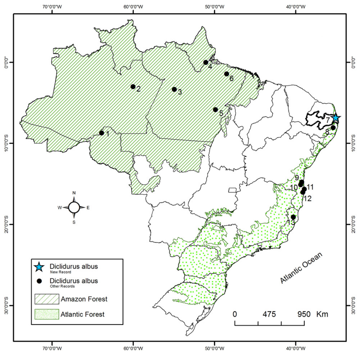
FIGURE 1. Distribution of Diclidurus albus in Brazil (star = new record; circles = existing records). Codes are as follows: 1: Porto Velho, RO (Peracchi et al. 2011); 2: Manaus, AM (Reis and Peracchi 1987, Bernard and Fenton 2002, Lim and Engstrom 2005, Peracchi et al. 2011, Bernard et al. 2011); 3: Floresta Nacional do Tapajós, PA (Castro-Arellano et al. 2007); 4: Tracajatuba, AP (Peracchi et al. 1984, Peracchi et al. 2011); 5: Floresta Nacional do Carajás, PA (Martins et al. 2012); 6: Belém, PA (Peracchi et al. 2011); 7: Rio Tinto, PB (this study); 8: Pernambuco State (Feijó and Langguth 2011); 9: Itabuna, BA (Faria et al. 2006); 10: Buerarema, BA (Vaz 2005); 11: Canavieiras, BA (Peracchi et al. 2011); 12: Rio Jequitinhonha, BA (Oliveira 2004); 13: Espírito Santo State (Mendes et al. 2010, Peracchi et al. 2011).
