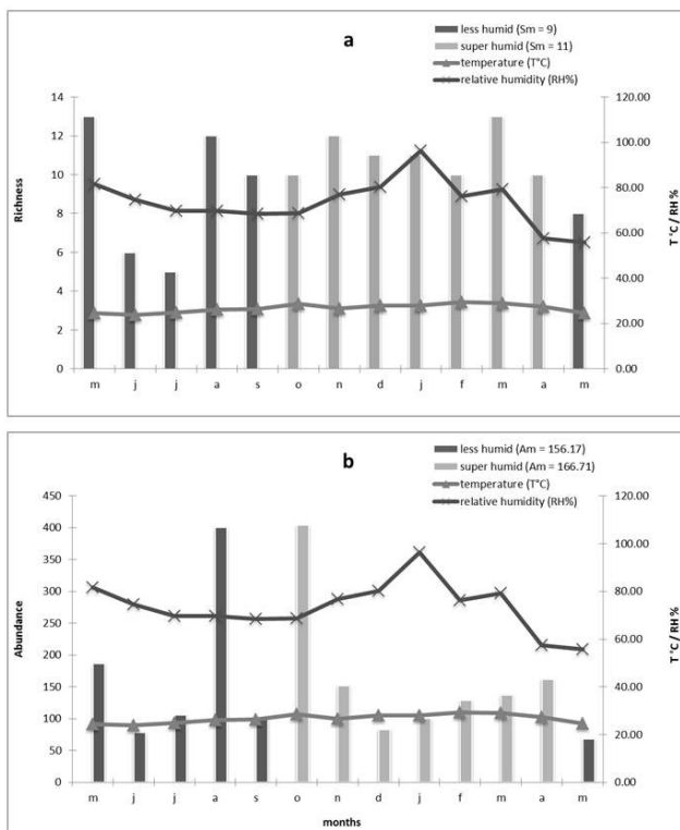
FIGURE 2. Diversity of social wasps related to temperature and relative humidity during the months of the year in Angelim Rainforest, Ubatuba, SP: (a) Richness of species ( S_m = average richness of each season) and (b) Abundance of species ( A_m = mean abundance of each).
