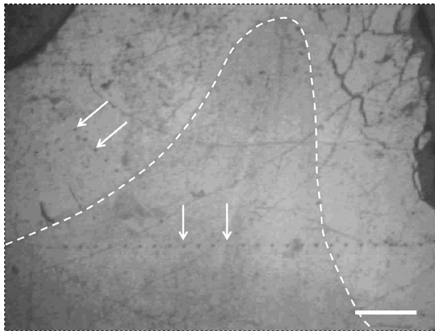
Figure 1. Polished slices of wild boar tooth tissue embedded in epoxy resin. The enamel-dentine junction (EDJ) is indicated by a dotted line. Some of the several marks of nano-indentation are indicated by arrows (scale bar = 200 \mu\text{m} ).
