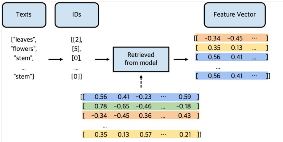
Figure 2. Embedding lookup retrieved from the language model.
