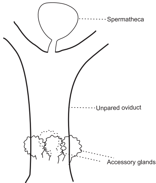
Figure 2. Schematic drawing of oviducts and spermatheca of studied Aclerda spp.
